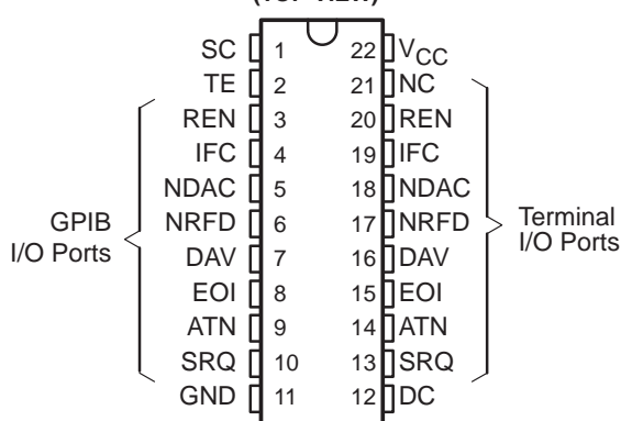
SN75162B . . . N PACKAGE (TOP VIEW)
