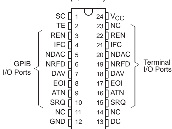
SN75162B . . . DW PACKAGE (TOP VIEW)
