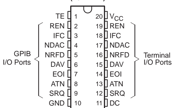
SN75161B . . . DW OR N PACKAGE (TOP VIEW)
