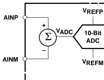
Figure 34. Differential Input Stage
