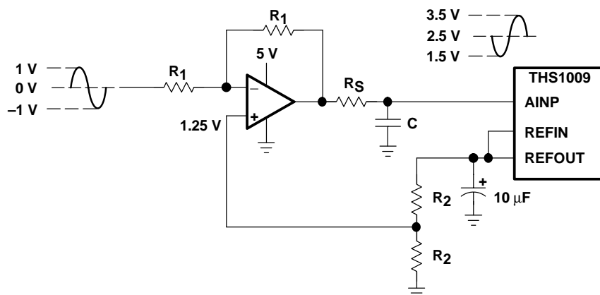
Figure 35. Level-Shift for DC-Coupled Input
