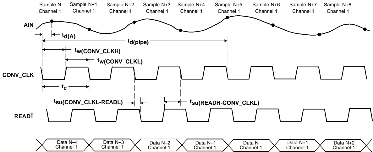
Figure 25. Conversion Timing in 1-Channel Operation
