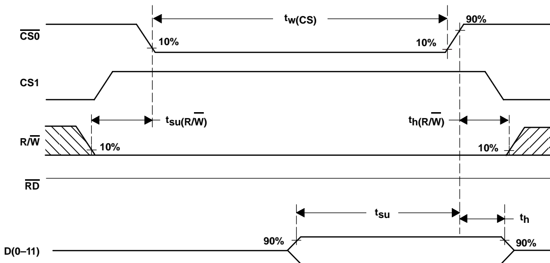
Figure 32. Write Timing Diagram Using \overline{R/W} ( \overline{CS0} -controlled)
