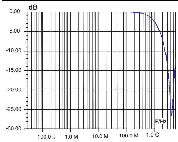
Figure 9. S21 attenuation measurement
