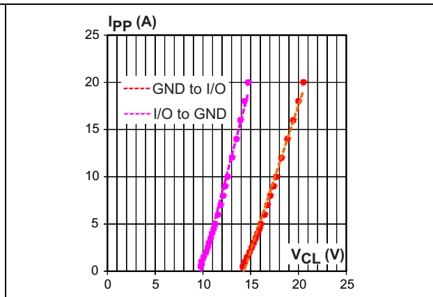
Figure 12. TLP measurement
