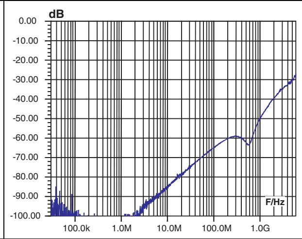
Figure 10. Analog crosstalk measurement
