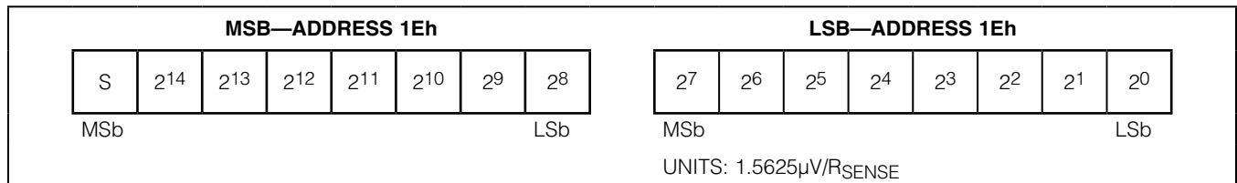
Figure 28. ICHGTerm Register Format (Input)
