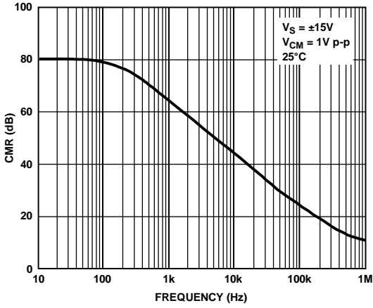
Figure 14. Common-Mode Rejection (CMR) vs. Frequency
