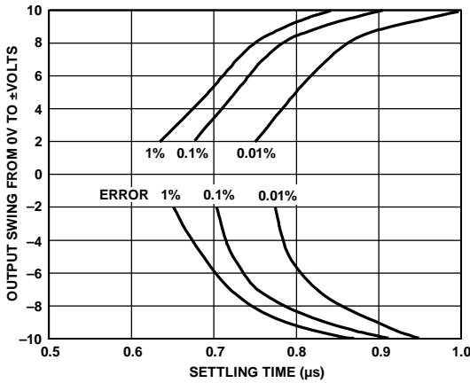
Figure 16. Output Swing and Error vs. Settling Time
