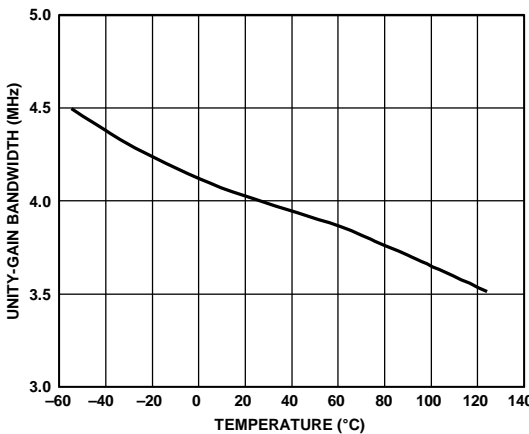
Figure 10. Unity-Gain Bandwidth vs. Temperature
