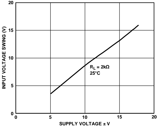
Figure 2. Input Voltage Swing vs. Supply Voltage
