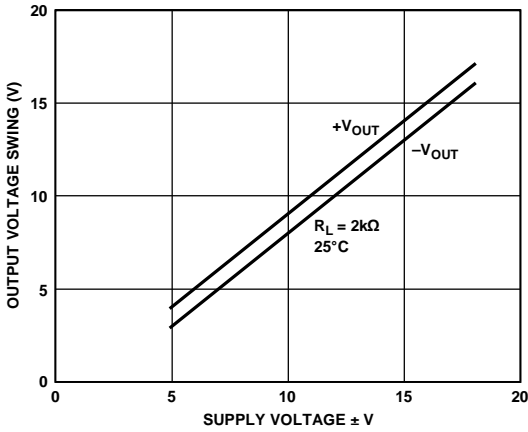
Figure 3. Output Voltage Swing vs. Supply Voltage
