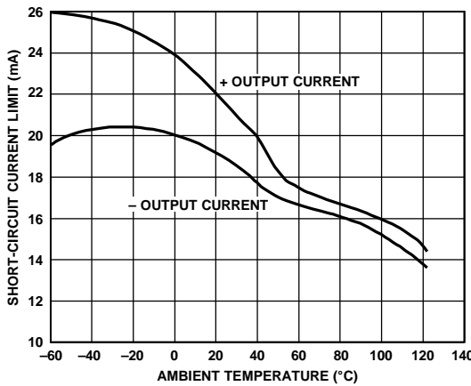
Figure 9. Short-Circuit Current Limit vs. Temperature
