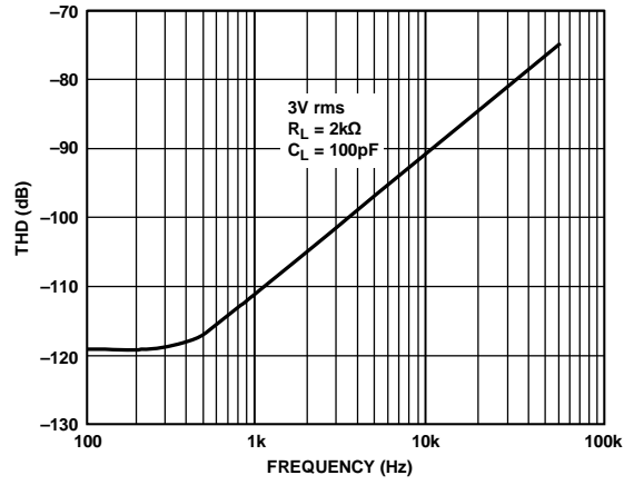
Figure 17. Total Harmonic Distortion (THD) vs. Frequency
