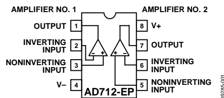
Figure 1. 8-Lead SOIC_N (R-Suffix)
