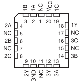
SN54HC11 ... FK PACKAGE (TOP VIEW)
