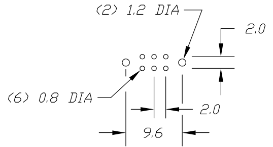
P.C.B. MOUNTING HOLES
