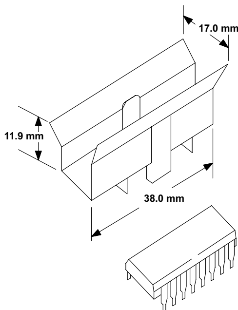
Figure 12. External Heat Sink Mounting Example ( \theta_{\text{JA}} = 25^\circ\text{C/W} )
