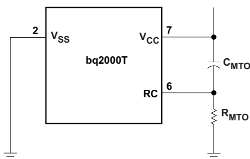
Figure 5. Typical Connection for the RC Input
