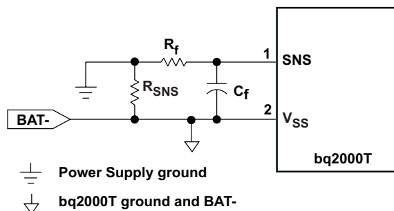
Figure 8. Current-Sensing Circuit
