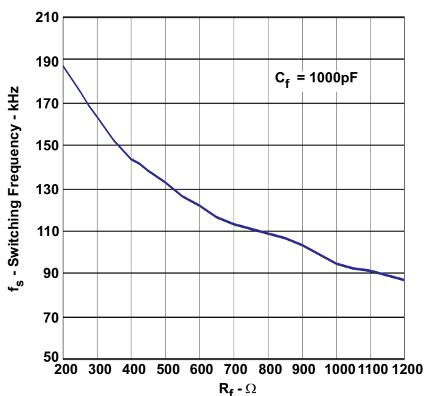
Figure 10. Switching Frequency vs Resistance
