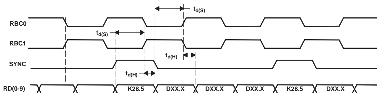
Figure 2. Synchronous Timing Characteristics Waveforms (TBI half-rate mode)
