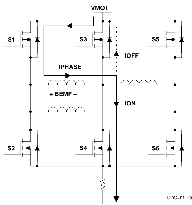
Figure 9. Two-Quadrant Chopping
