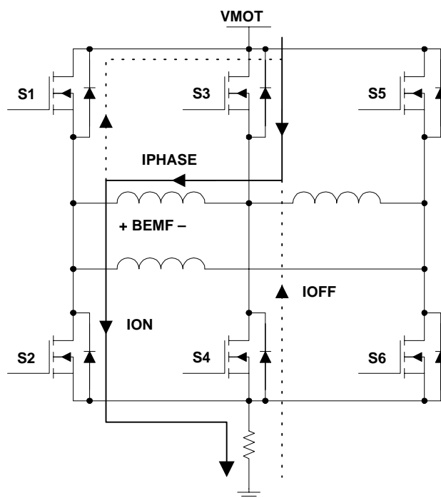
Figure 11. Four-Quadrant Reversal
