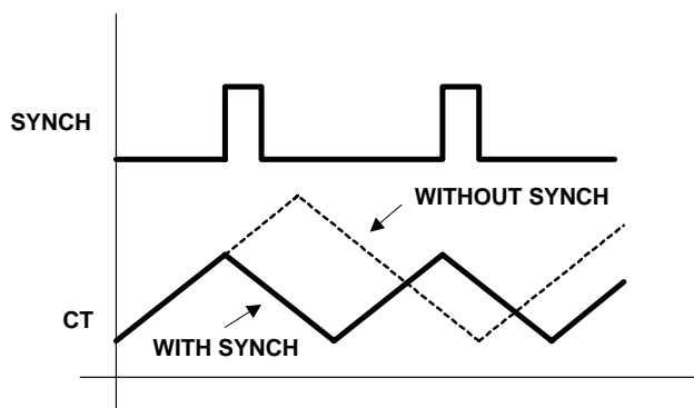
Figure 4. Oscillator Waveforms
