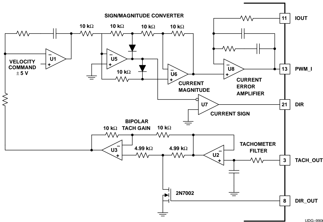
Figure 16. Four-Quadrant Control Loop
