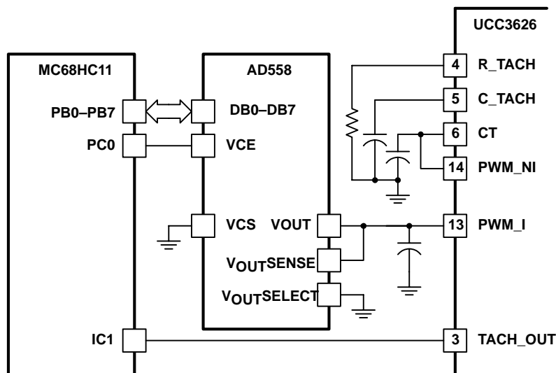
Figure 6. Digital Velocity Loop Implementation Using MC68HC11
