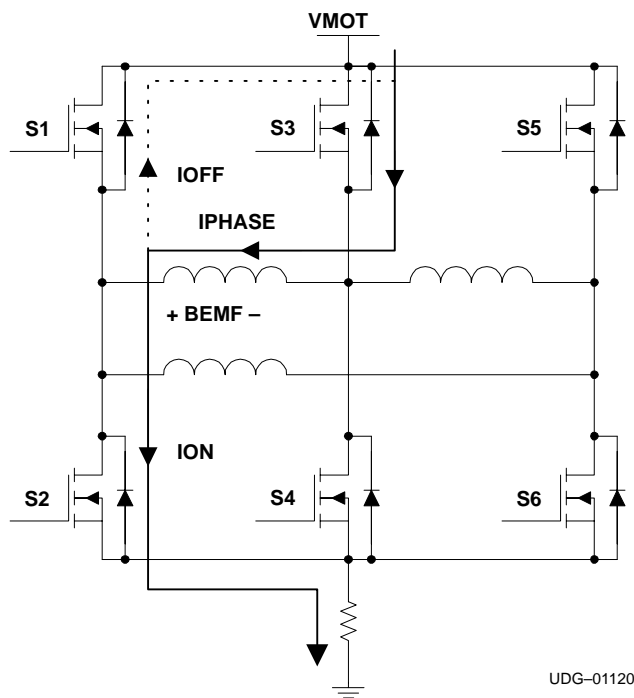
Figure 10. Two-Quadrant Reversal
