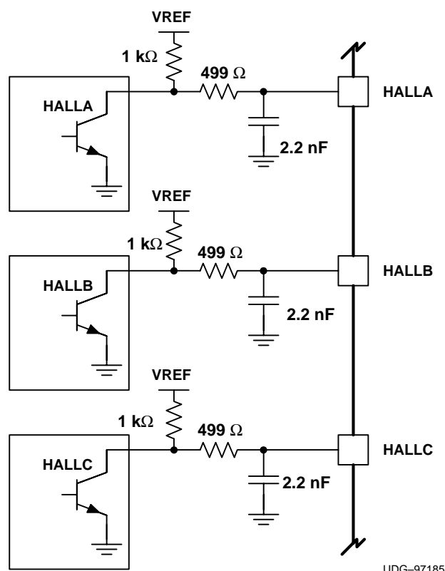
Figure 2. Passive Hall Filtering Technique
