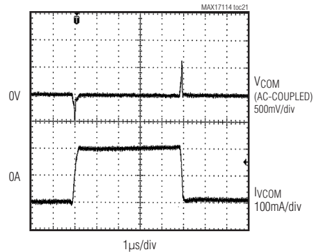
OPERATIONAL AMPLIFIER LOAD-TRANSIENT RESPONSE
