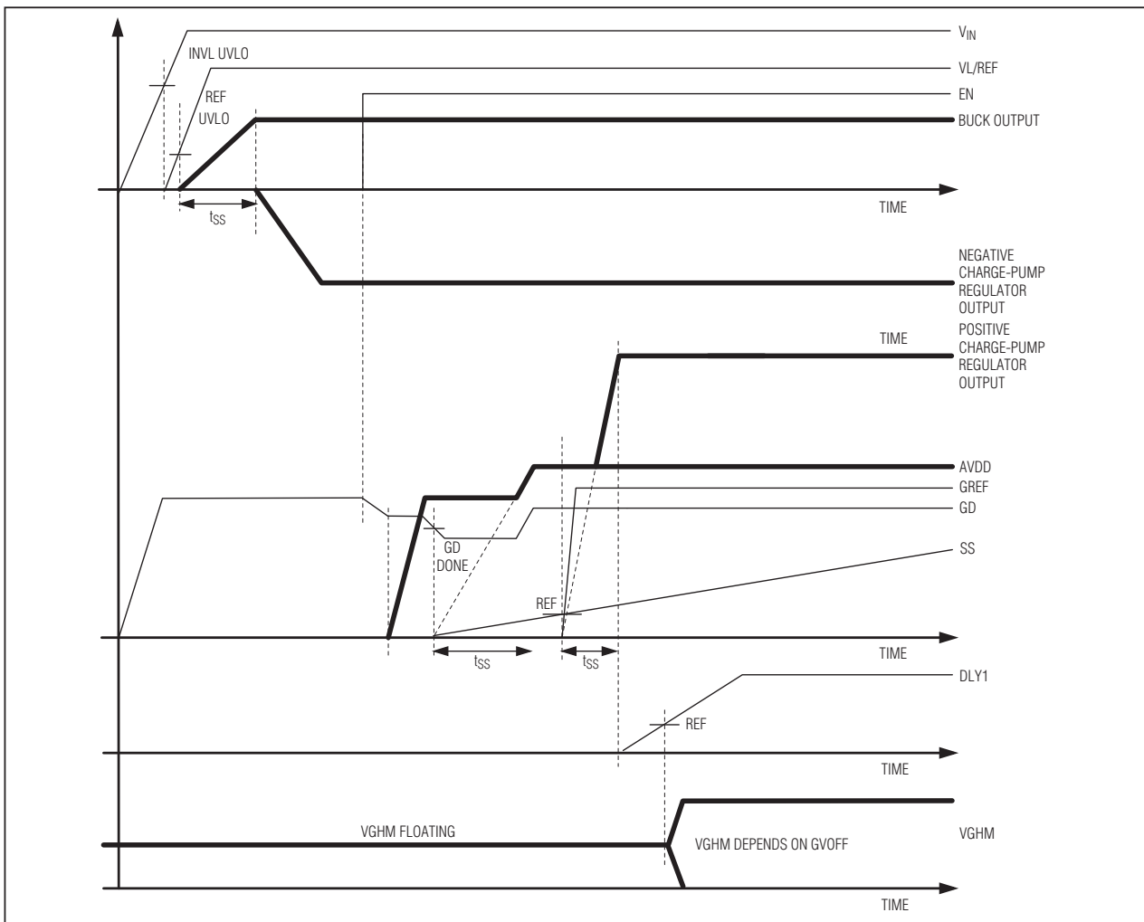
Figure 7. Power-Up Sequence
