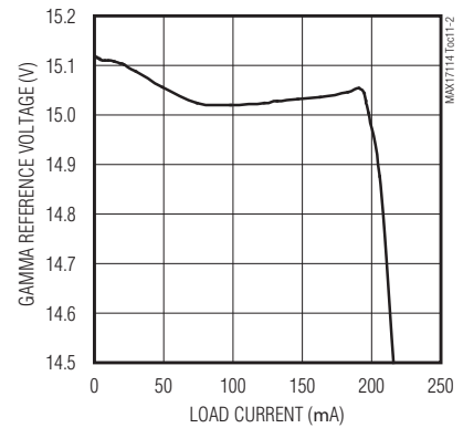
GAMMA REFERENCE LOAD REGULATION ( V_{REF} = 16V )
