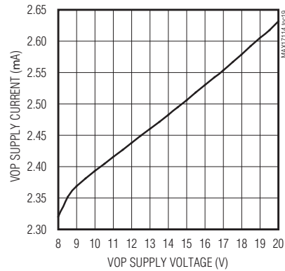
OPERATIONAL AMPLIFIER SUPPLY CURRENT vs. SUPPLY VOLTAGE
