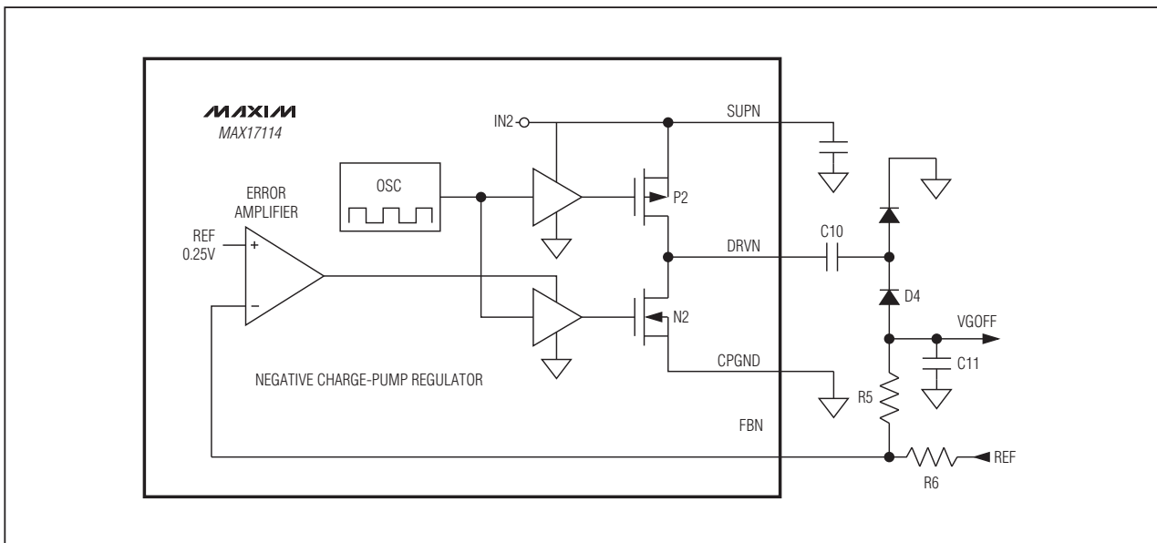
Figure 4. Negative Charge-Pump Regulator Block Diagram
