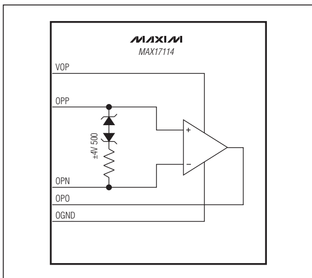
Figure 6. Op Amp Input Clamp Structure
