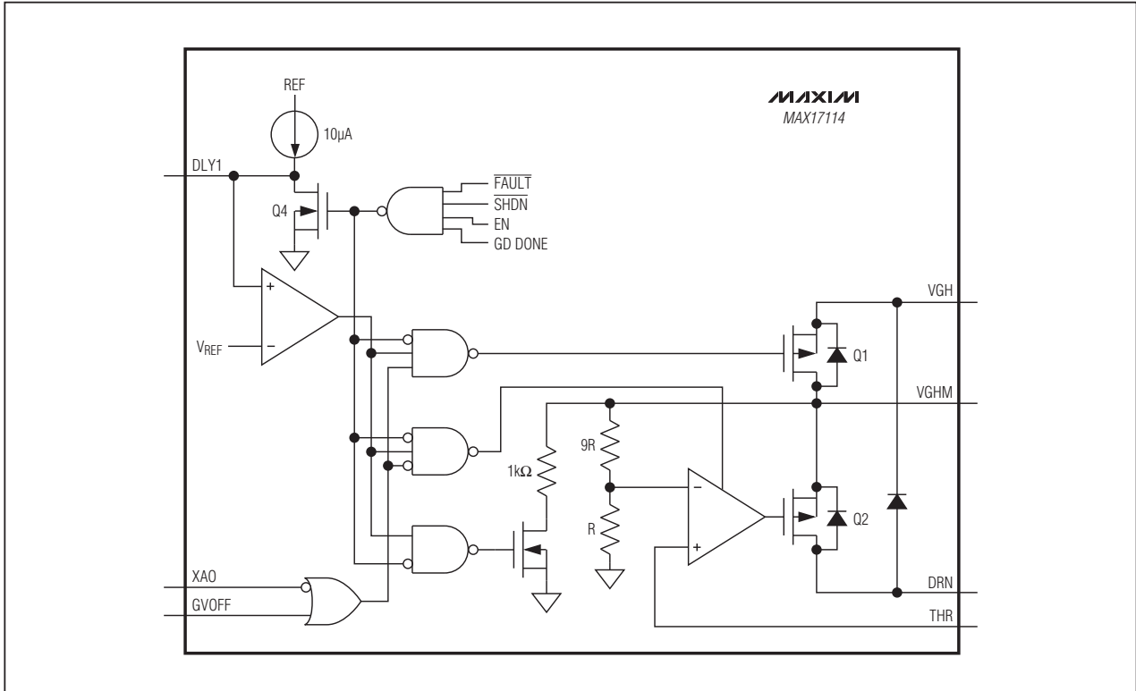
Figure 5. Switch Control
