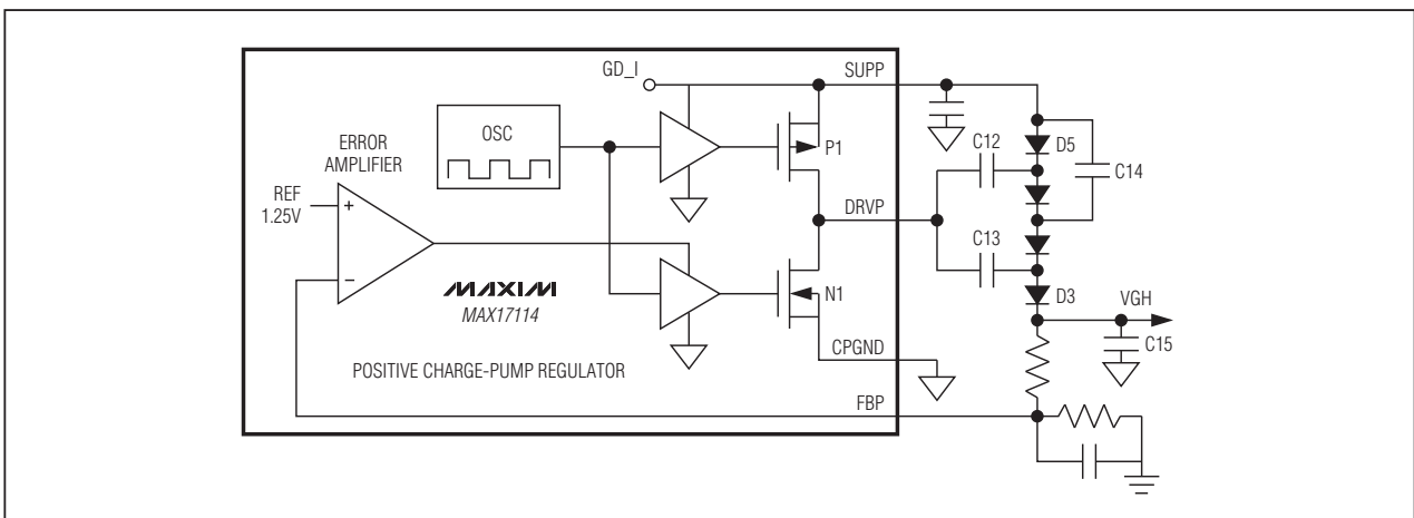
Figure 3. Positive Charge-Pump Regulator Block Diagram
