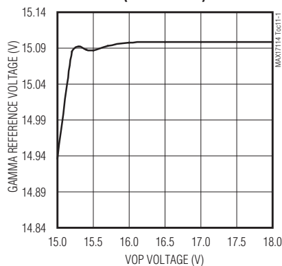
GAMMA REFERENCE LINE REGULATION (LOAD = 20mA)
