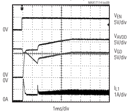
STEP-UP REGULATOR HEAVY LOAD SOFT-START (0.5A)
