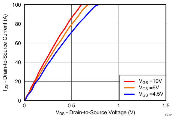
Figure 3. Saturation Characteristics
