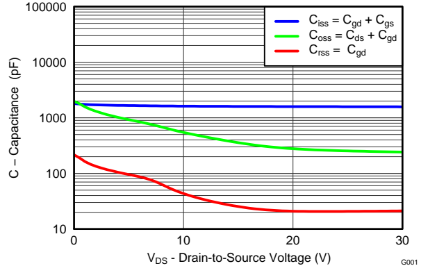
Figure 6. Capacitance
