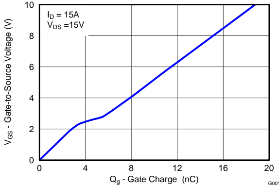
Figure 5. Gate Charge
