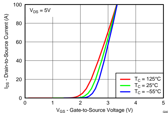
Figure 4. Transfer Characteristics
