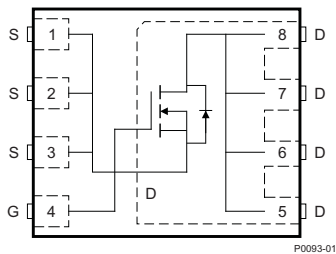
Figure 1. Top View
