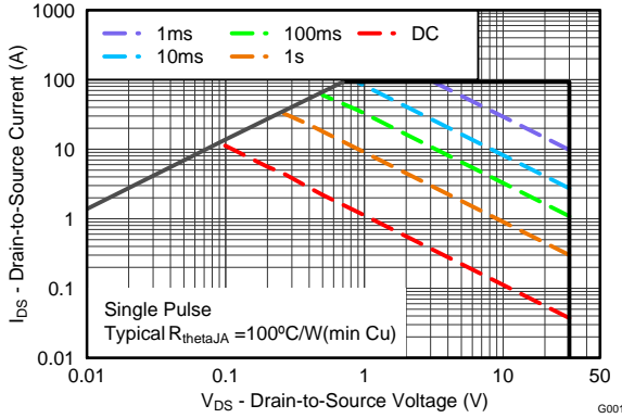
Figure 11. Maximum Safe Operating Area
