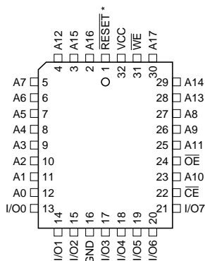
PLCC Top View
