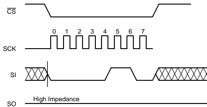
Figure 7. Write Enable Latch Sequence
