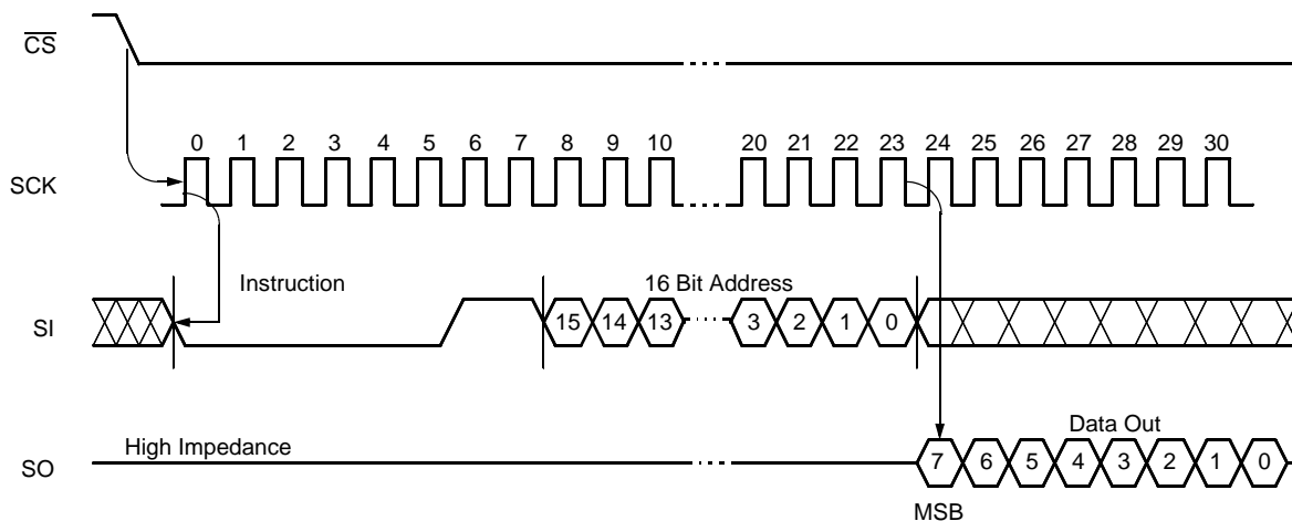
Figure 5. Read EEPROM Array Sequence
