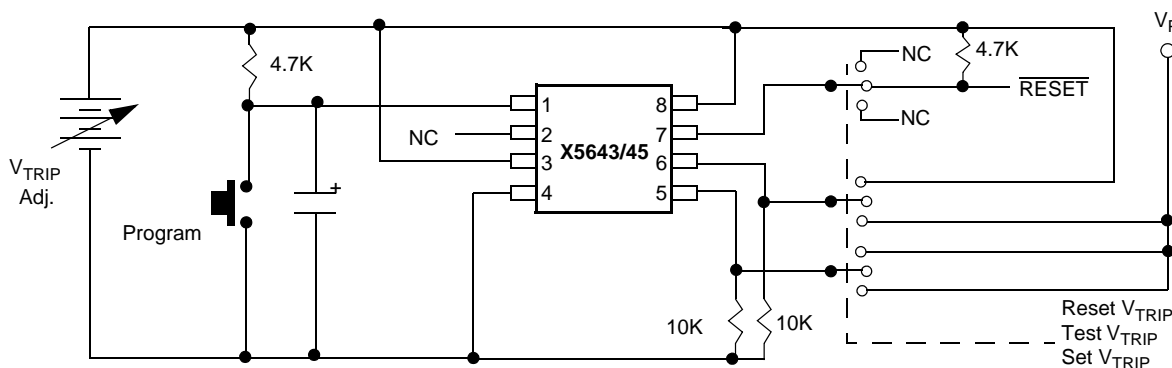
Figure 4. Sample V TRIP Reset Circuit
