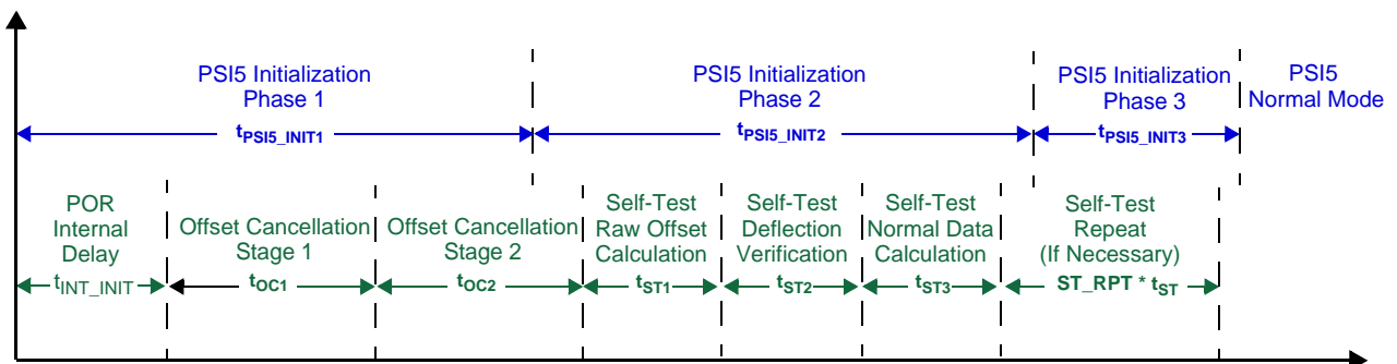
Figure 25. Initialization Timing
