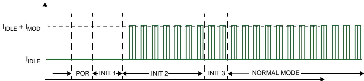
Figure 24. PSI5 Sensor 10-Bit Initialization
