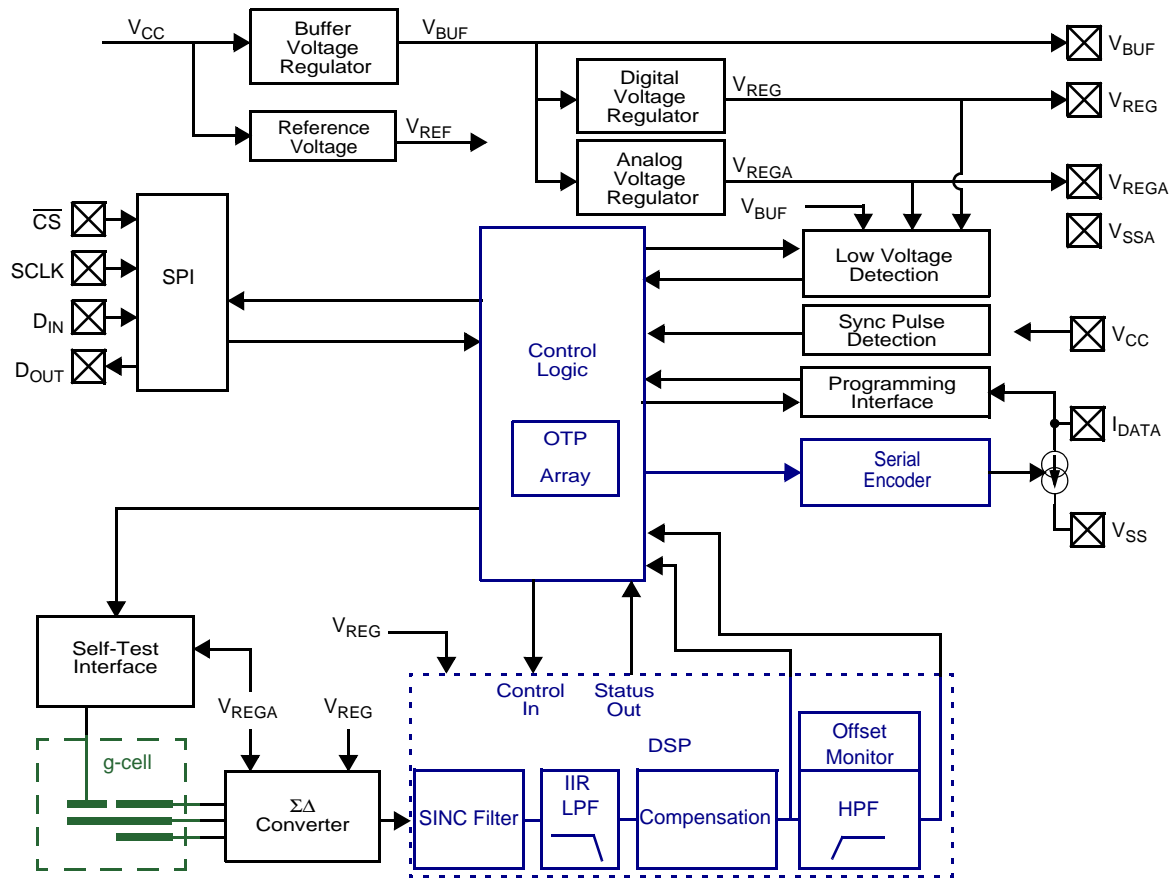
Figure 3. Block Diagram
