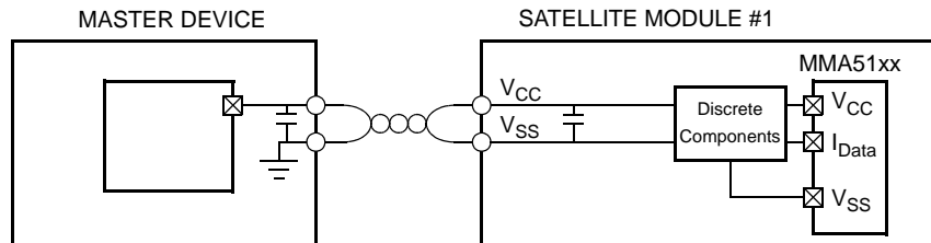
Figure 21. PSI5 Satellite Interface Diagram
