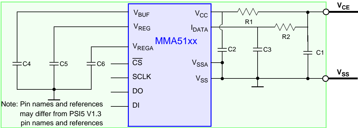
Figure 1. Application Diagram
