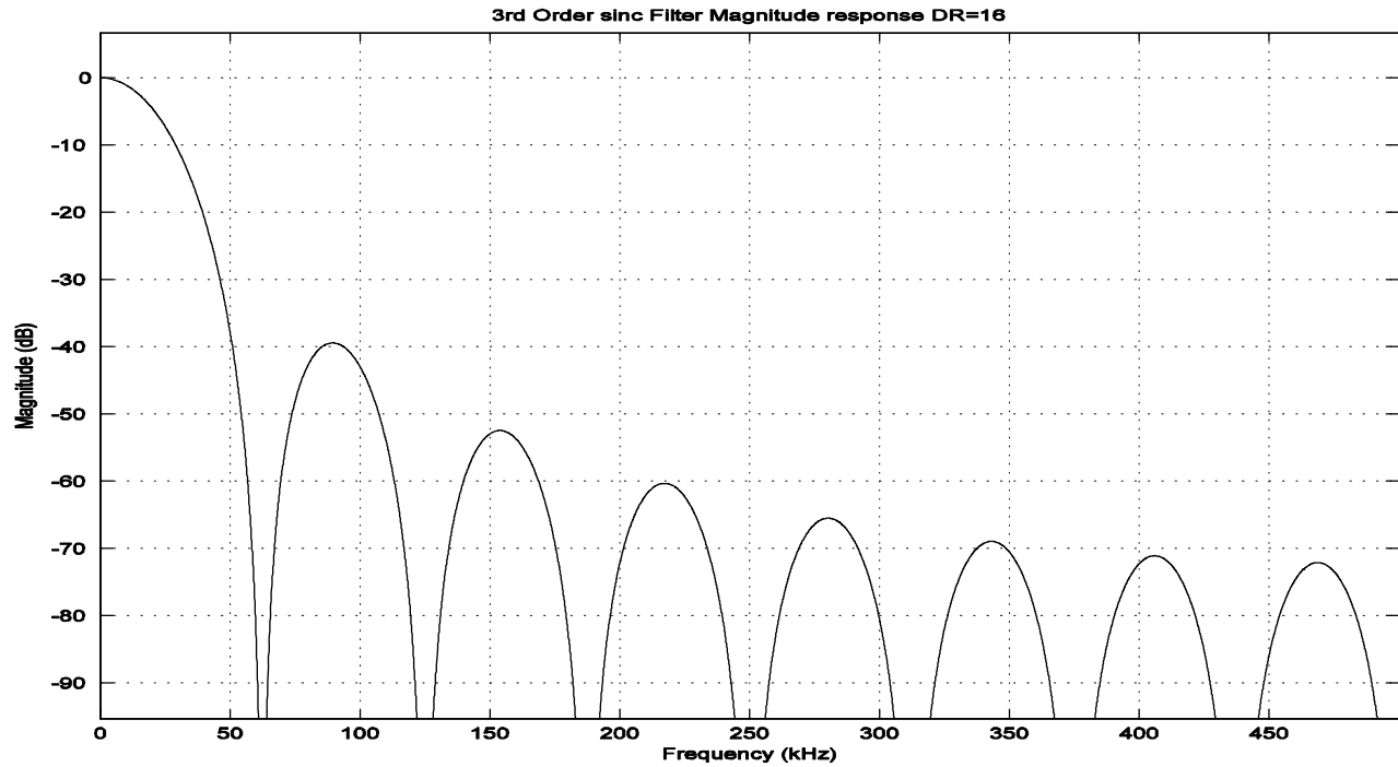
Figure 14. Sinc Filter Response, t_s = 16 \mu s
