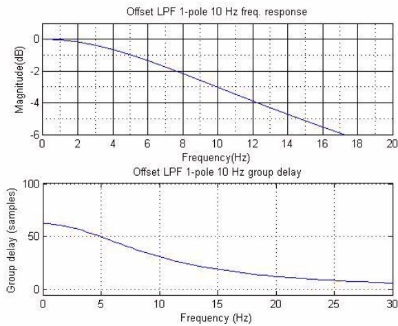
Figure 17. 10 Hz Offset Cancellation Low-Pass Filter Characteristics
