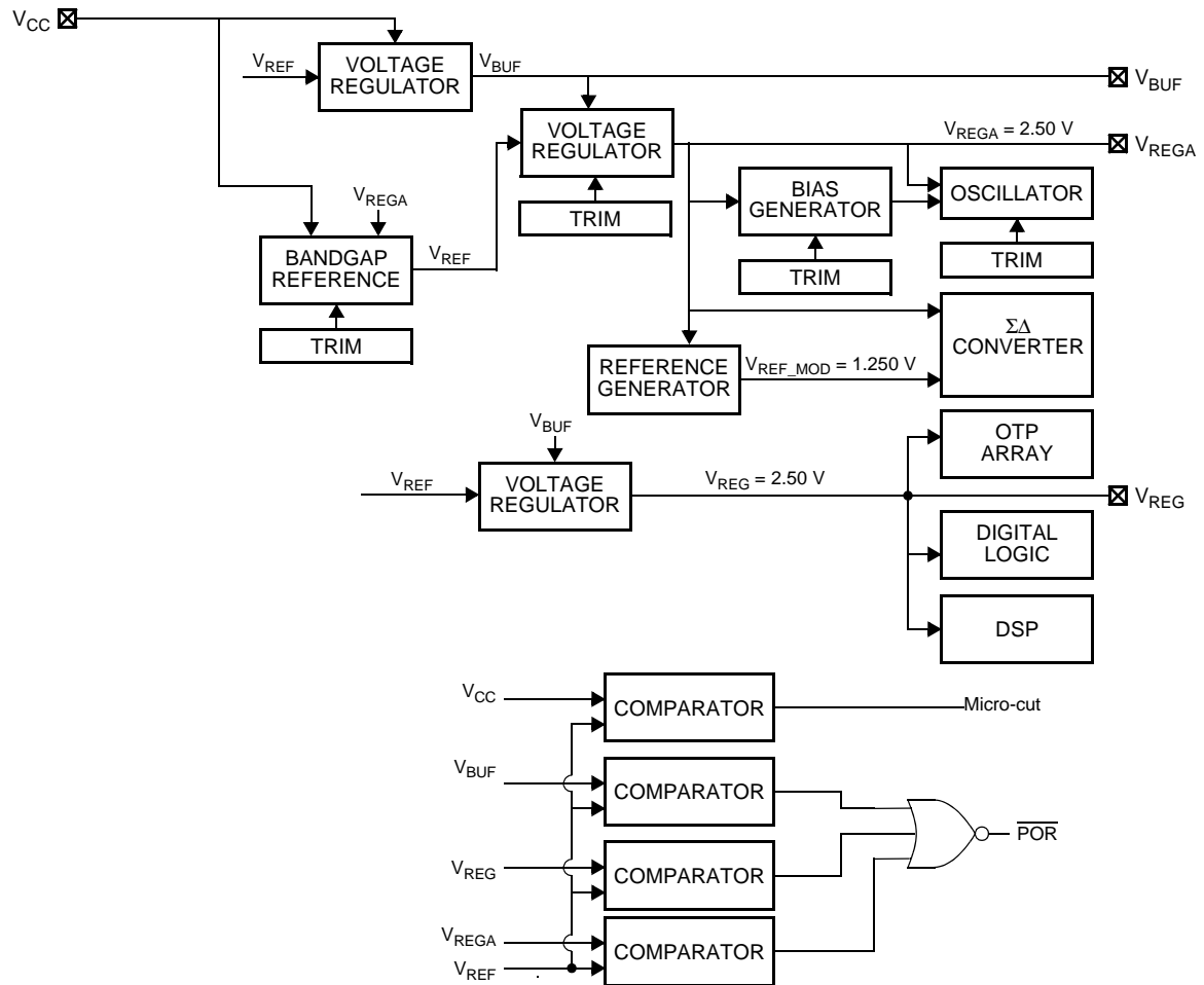
Figure 7. Voltage Regulation and Monitoring
