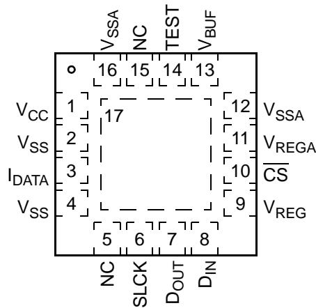
Figure 4. Top View, 16-Pin QFN Package
