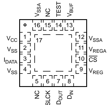
PIN CONNECTIONS
