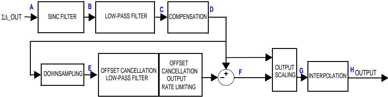
Figure 13. Signal Chain Diagram
