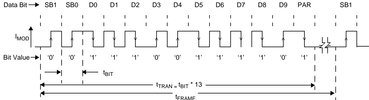
Figure 23. Example Manchester Encoded Data Transfer - PSI5-x10P
