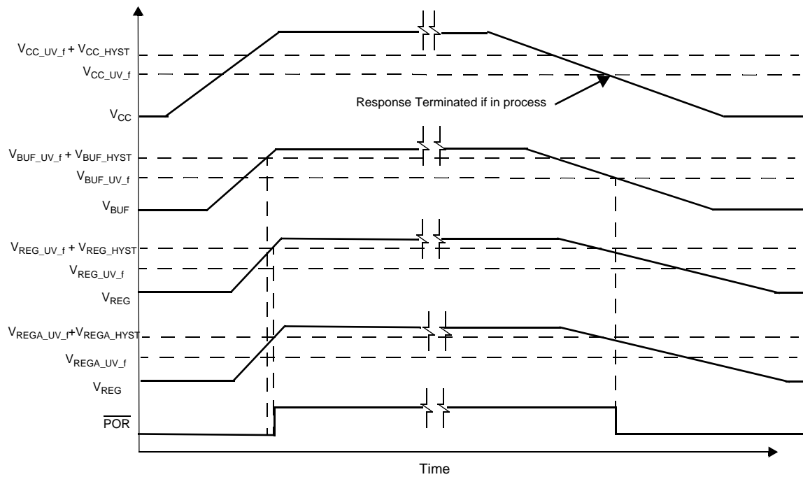
Figure 5. Powerup Timing
