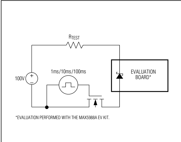
Figure 1. MAX5991A/MAX5991B Internal TVS Test Setup
