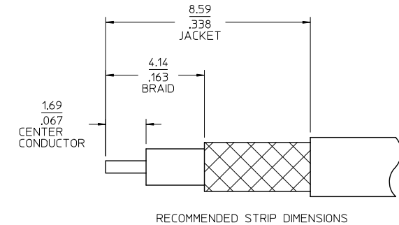
RECOMMENDED STRIP DIMENSIONS
