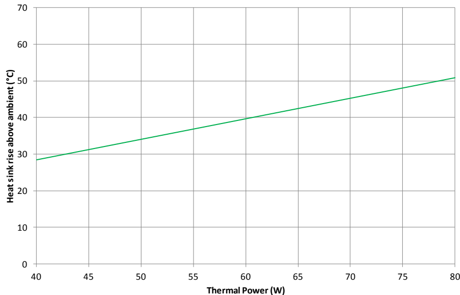
Heatsink Rise Above Ambient vs. Thermal Power Round Heatsinks Diameter 150 mm
