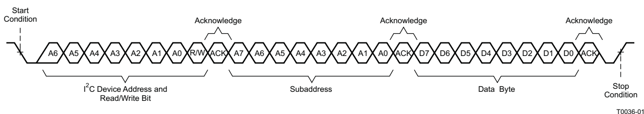
Figure 17. Random-Write Transfer
