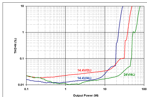
Figure 3. THD+N vs BTL Output Power at 1kHz
