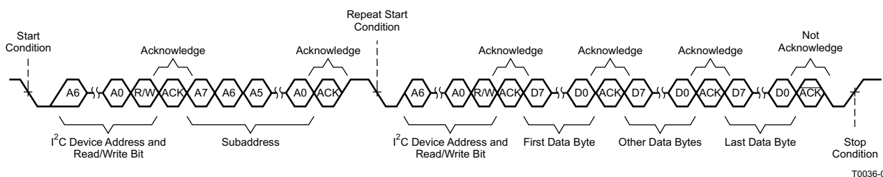
Figure 20. Sequential Read Transfer
