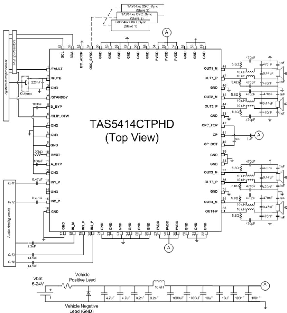
Figure 21. TAS5414C-Q1 Typical Application Schematic
