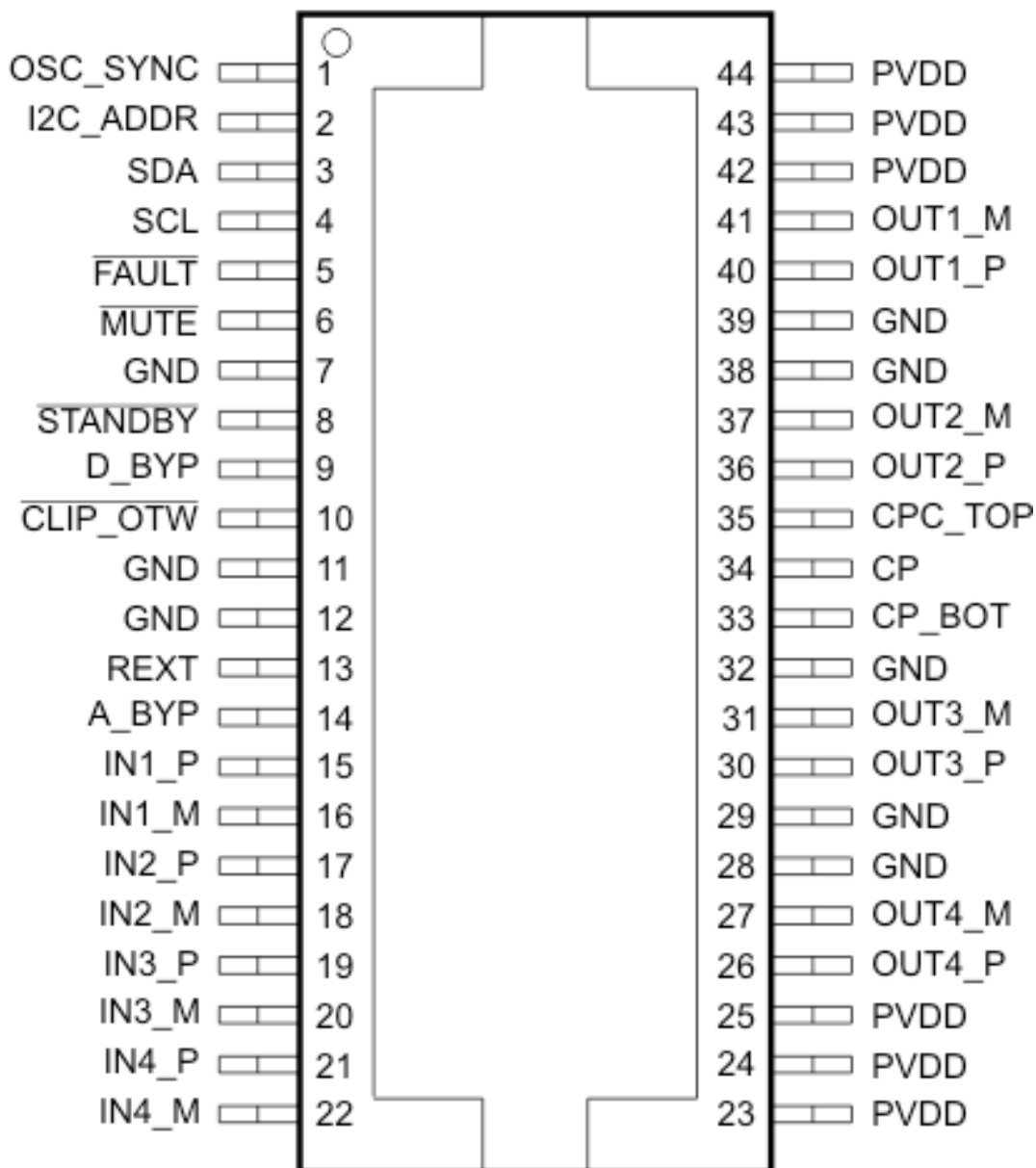
DKE Package (Top View)
