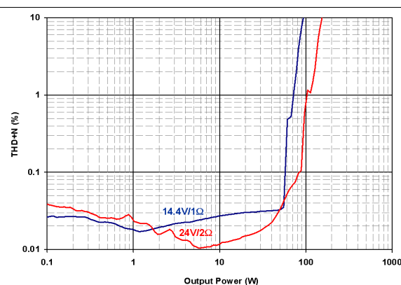
Figure 4. THD+N vs PBTl Output Power at 1kHz
