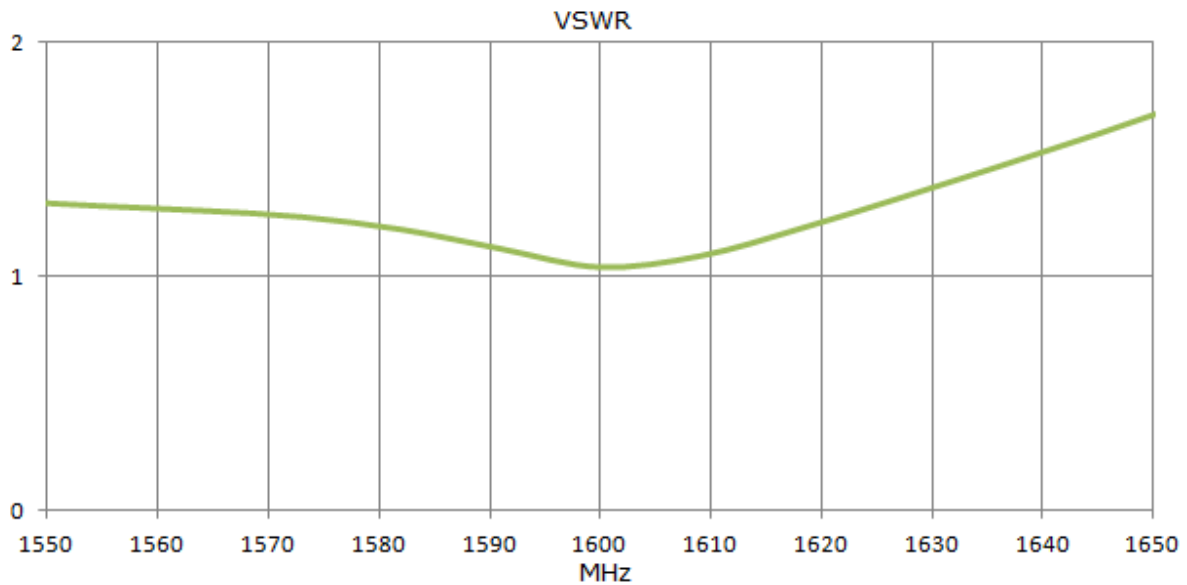
Figure 3: VSWR of FXP611 GPS/GLONASS/COMPASS Antenna
