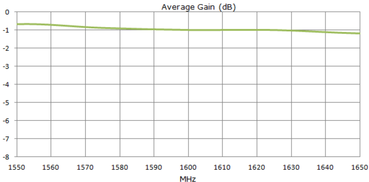
Figure 6: Average Gain of FXP611 GPS/GLONASS/COMPASS Antenna
