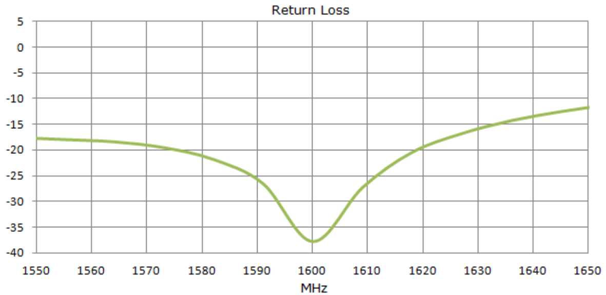
Figure 2: Return loss of FXP611 GPS/GLONASS/COMPASS Antenna
