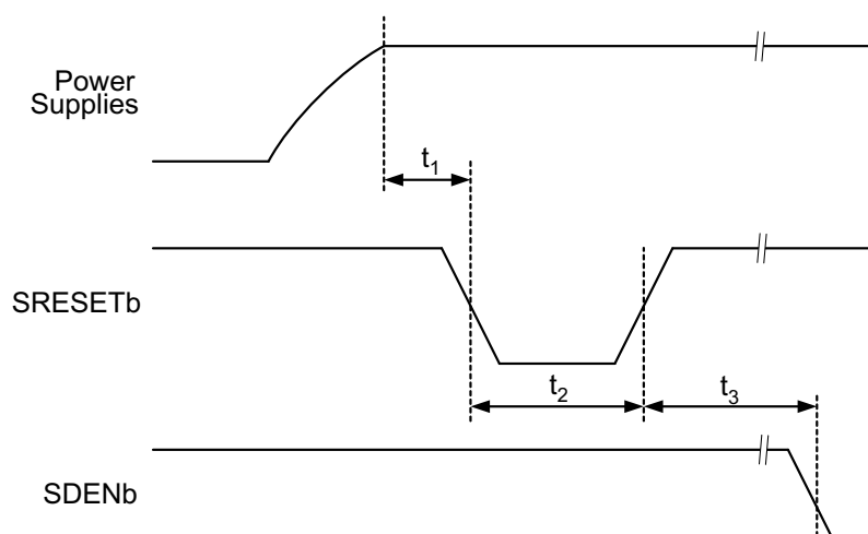
Figure 38. Device Initialization Timing Diagram
