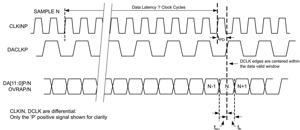
Figure 3. Timing Diagram for 12-bit DDR Output
