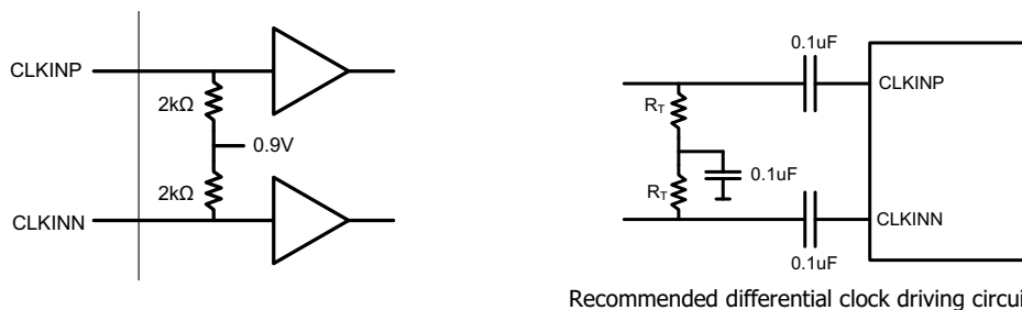
Figure 35. Recommended Differential Clock Driving Circuit
