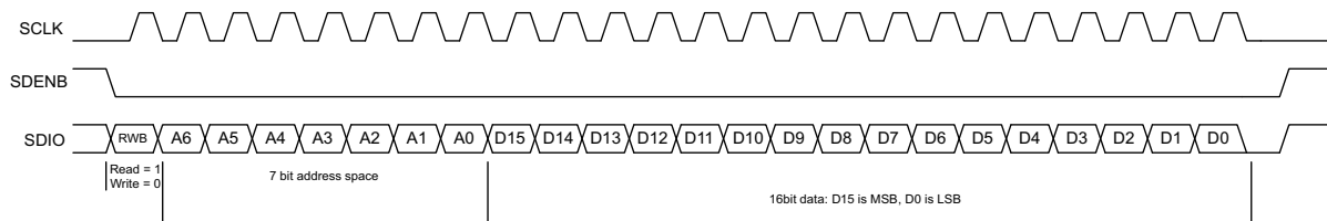
Figure 39. Serial Register Write Timing Diagram
