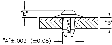
TYPICAL ASSEMBLY
