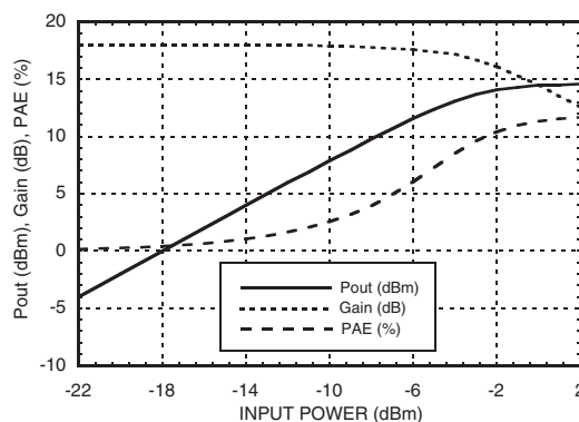
Power Compression @ 3 GHz
