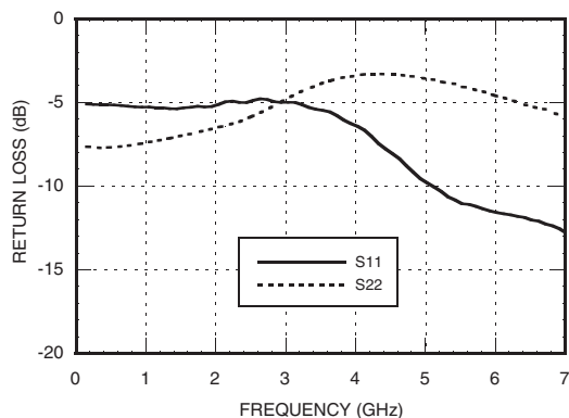
Input & Output Return Loss
