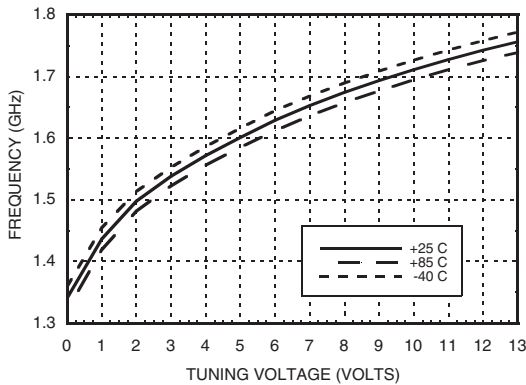
Divide-by-16 Frequency vs. Tuning Voltage, Vcc = +5V
