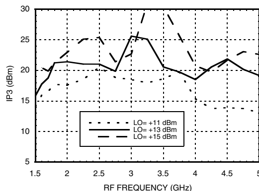
Single Channel: Upconverter IP3 vs. LO Drive
