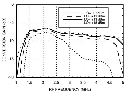
Single Channel: Conversion Gain vs. LO Drive
