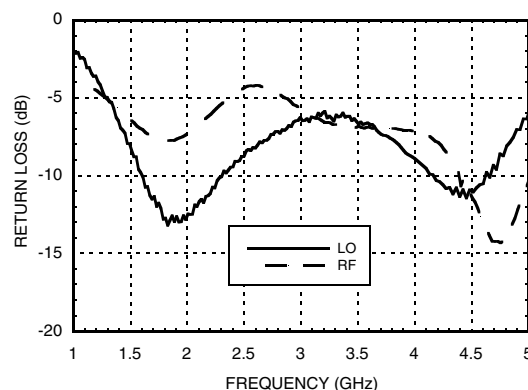
Single Channel: Return Loss @ LO = +13 dBm
