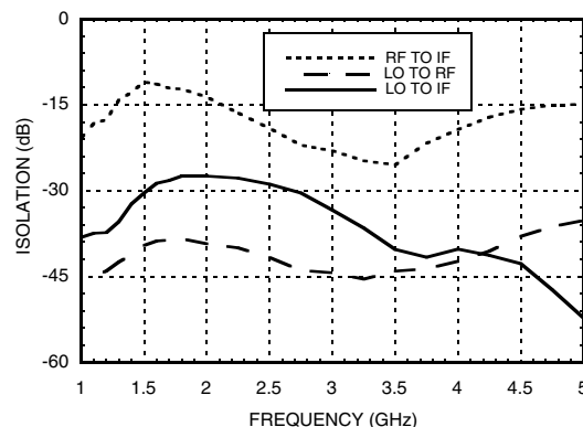
Single Channel: Isolation @ LO = +13 dBm
