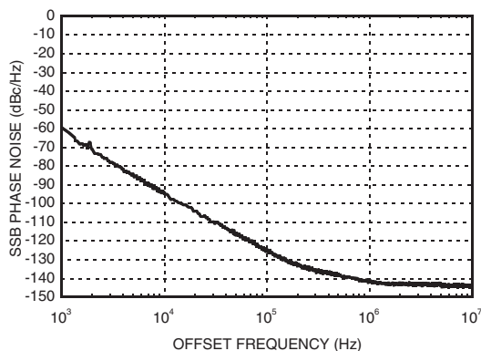
Divided Output SSB Phase Noise @ Vtune = 5V
