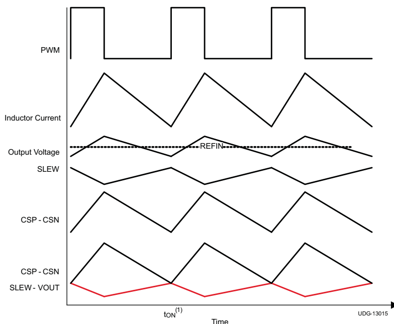
Figure 30. On-Time Waveforms (1)
