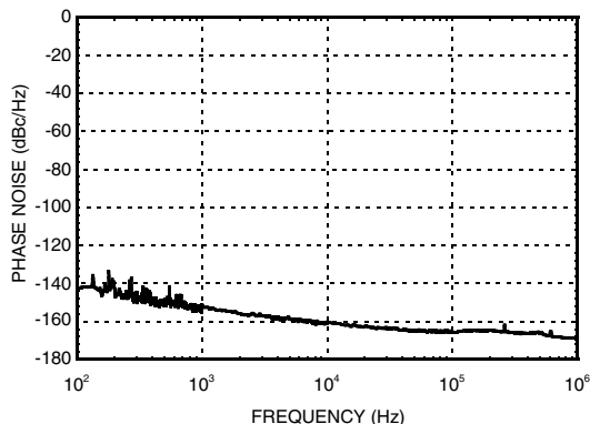
Phase Noise at P1dB @ 12 GHz
