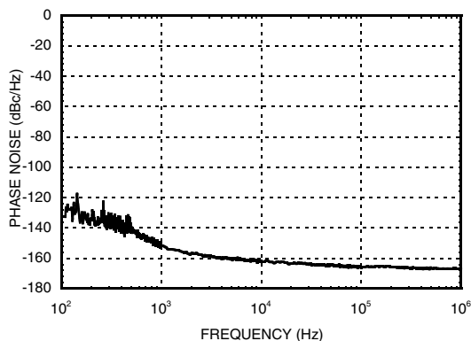
Phase Noise at Psat @ 2 GHz
