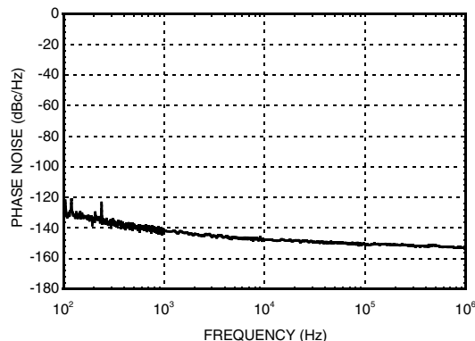
Phase Noise at P1dB @ 18 GHz
