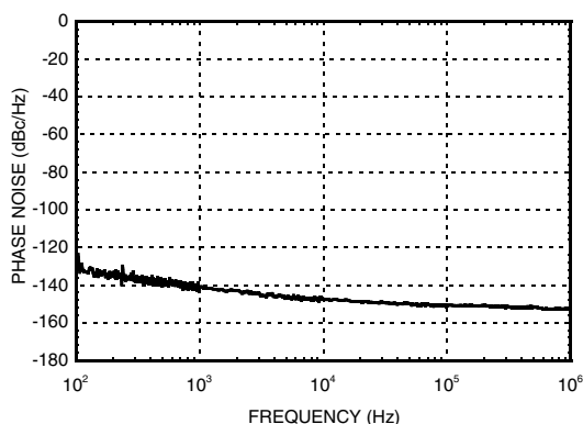
Phase Noise at Psat @ 18 GHz
