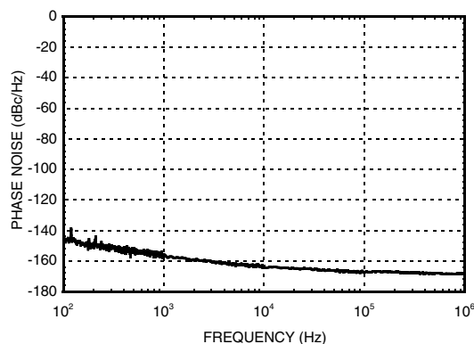
Phase Noise at P1dB @ 2 GHz
