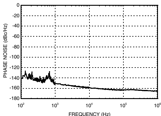
Phase Noise at Pout = 0 dBm @ 12 GHz
