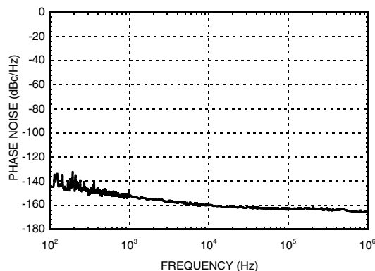
Phase Noise at Psat @ 12 GHz
