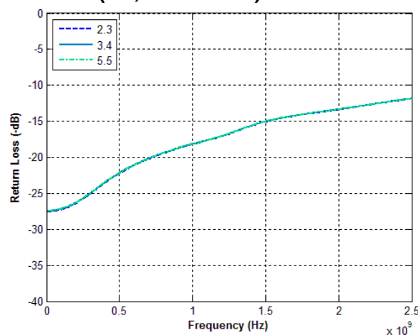
Figure 16. Return Loss vs. V_{DD} (RX, Attenuated)
