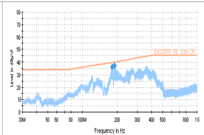
Figure 15: test result(Horizontal)
