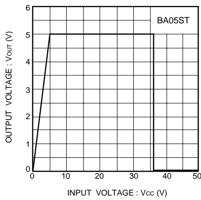
Fig.11 Over voltage protection characteristics
