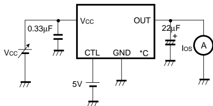
Fig.5 Measurement circuit for output short-circuit current
