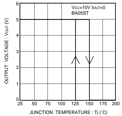
Fig.9 Thermal cutoff circuit characteristics
