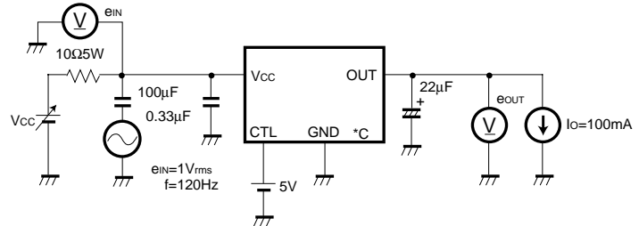
Fig.2 Measurement circuit for ripple rejection ratio
