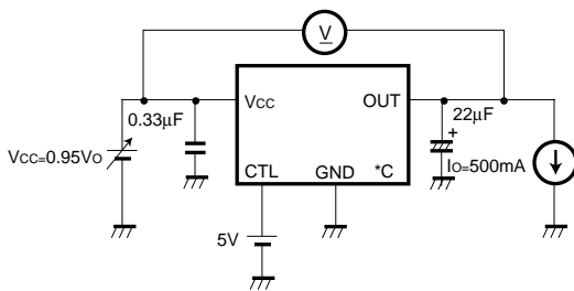
Fig.3 Measurement circuit for minimum I/O voltage differential
