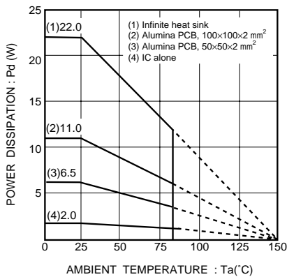
Fig. 7 Thermal derating curves (TO220FP-5)
