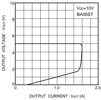
Fig.10 Current limit characteristics
