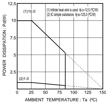
Fig.8 Thermal derating curves (TO252-5)
