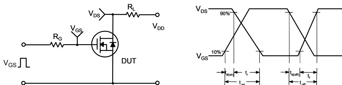
Figure 22. Resistive Switching Test Circuit & Waveforms
