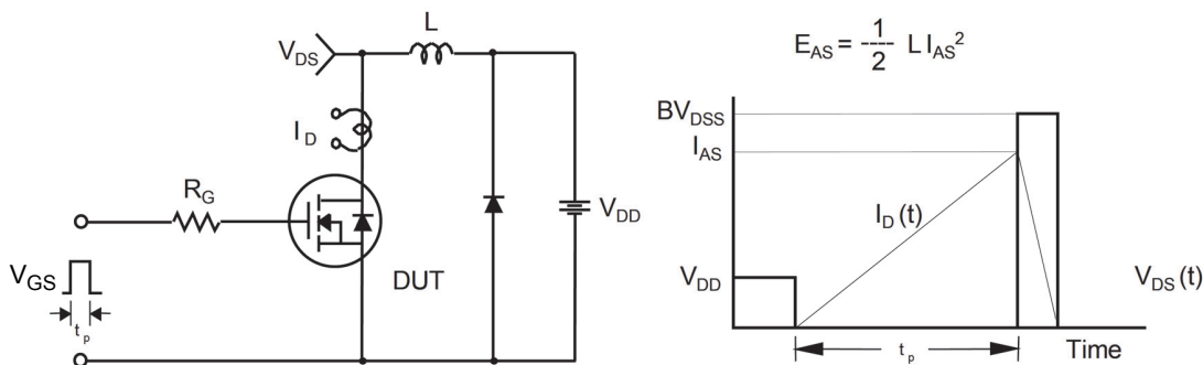
Figure 23. Unclamped Inductive Switching Test Circuit & Waveforms
