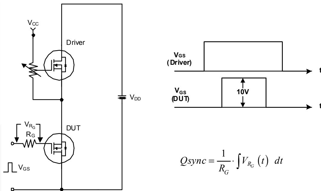
Figure 25. Total Gate Charge Q_{sync} . Test Circuit & Waveforms
