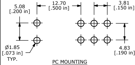
PC MOUNTING
