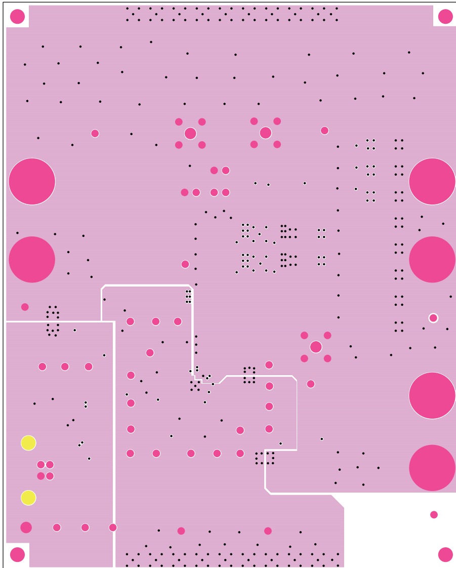
FIGURE 11. LAYER 3 COPPER
