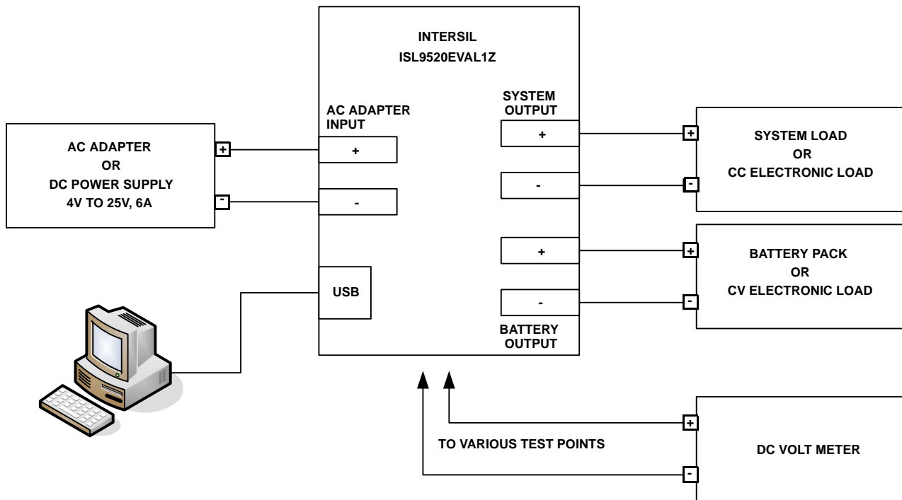
FIGURE 1. ISL9520EVAL1Z HARDWARE CONNECTION DIAGRAM
