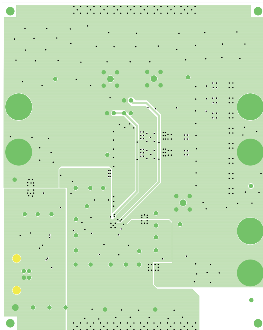
FIGURE 10. LAYER 2 COPPER
