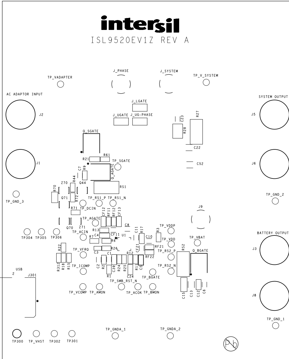
FIGURE 7. TOP SILKSCREEN
