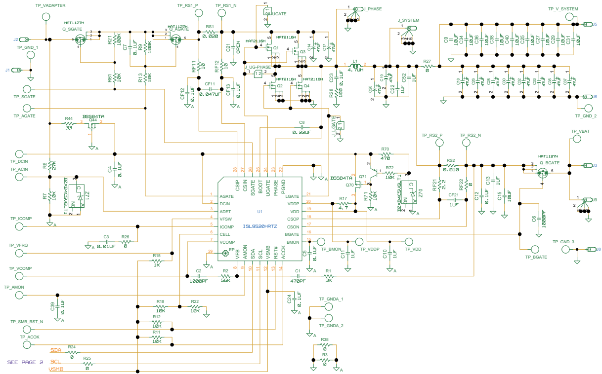
FIGURE 5. ISL9520EVAL1Z REV A SCHEMATIC
