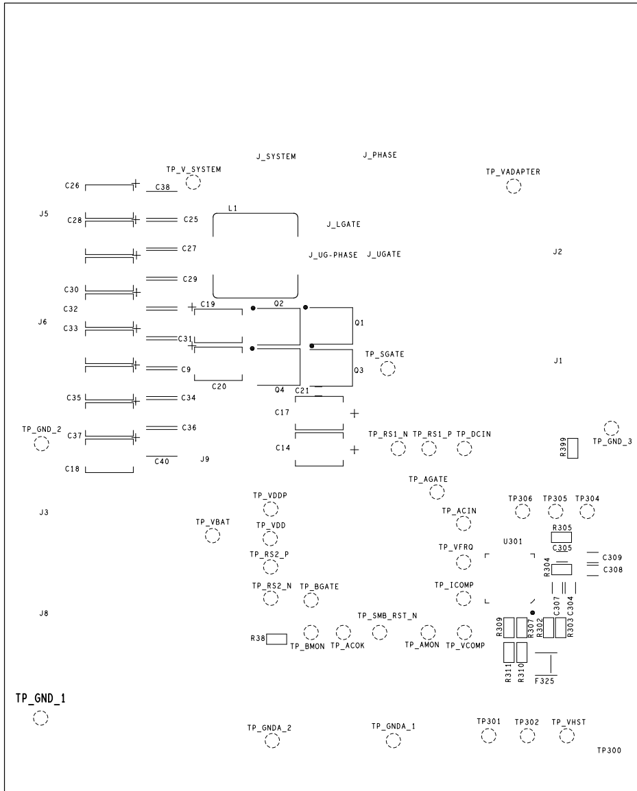
FIGURE 8. BOTTOM SILKSCREEN
