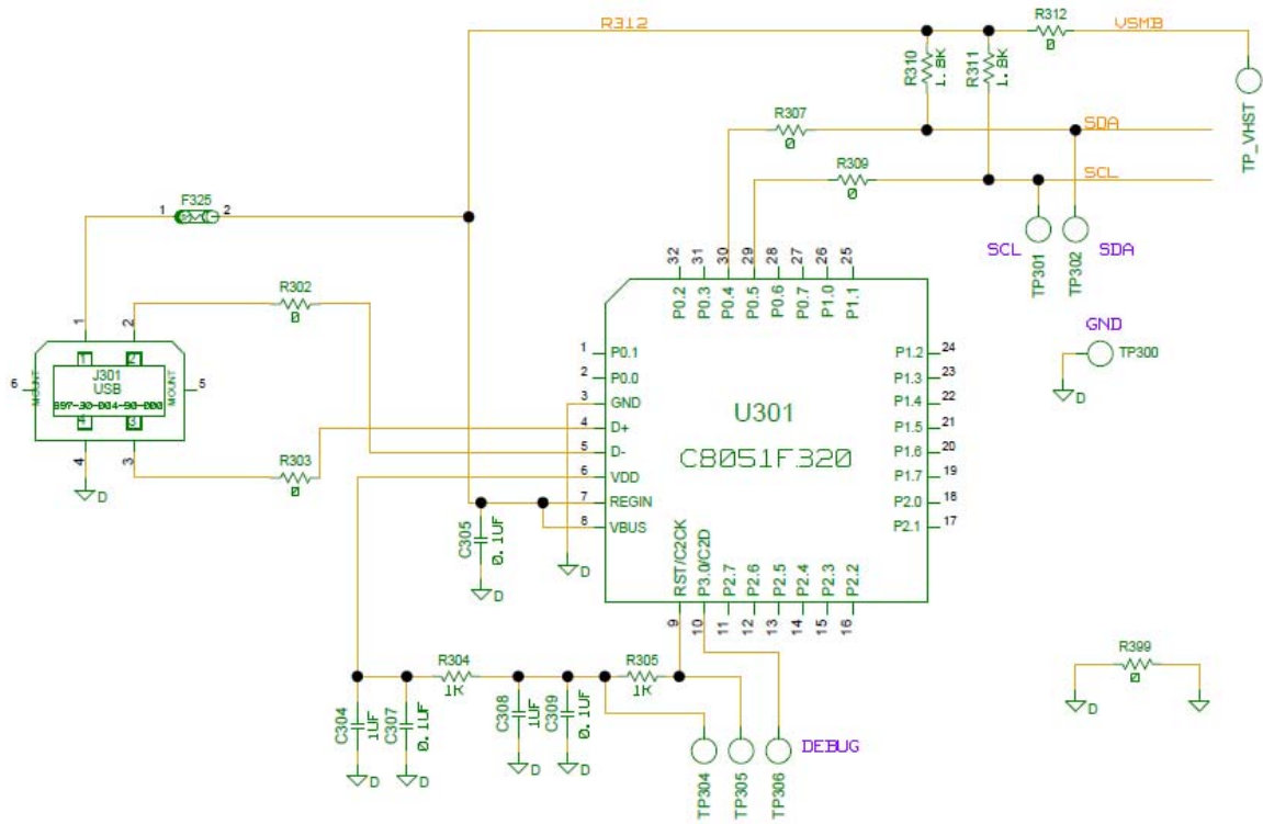
FIGURE 6. ISL9520 EVAL1Z REV A SCHEMATIC
