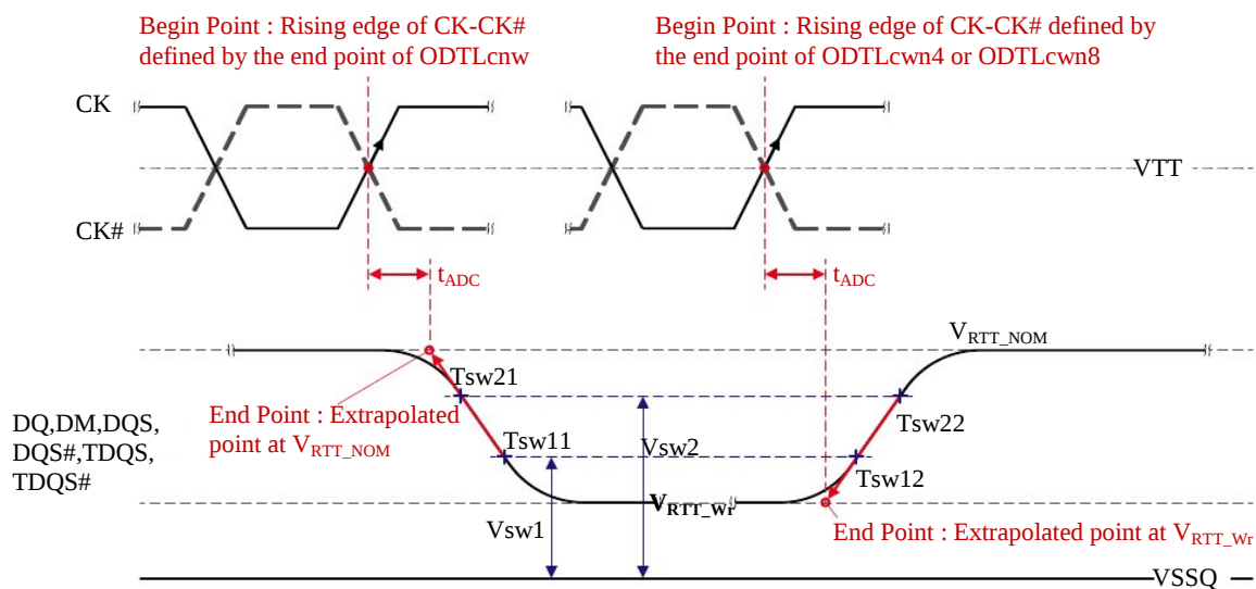
Figure 5.9.2.5 Definition of t_{ADC}
