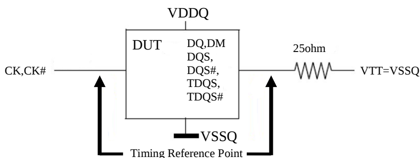
Figure 5.9.1 ODT Timing Reference Load
