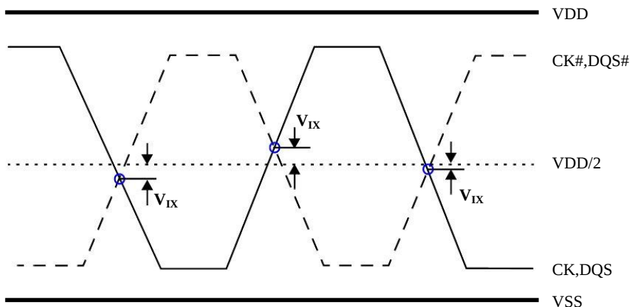
Figure 4.4. V_{IX} Definition
