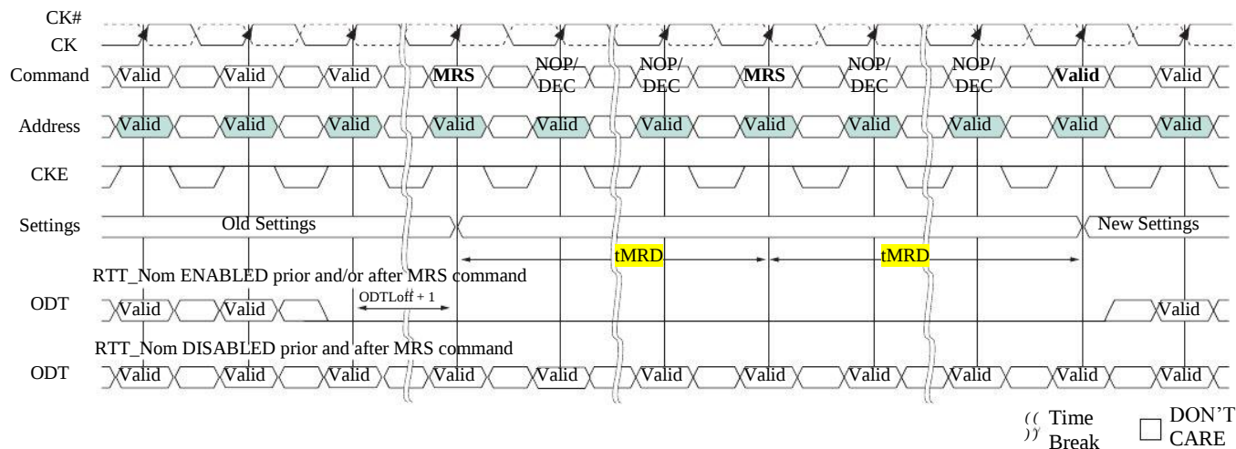
Figure 2.3.1a tMRD Timing
