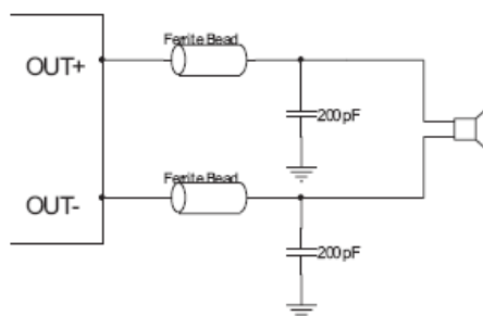
Figure 3. Ferrite Bead Filter to reduce EMI
