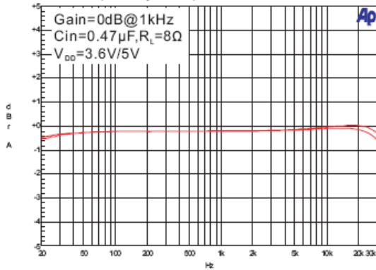
7. Frequency Response
