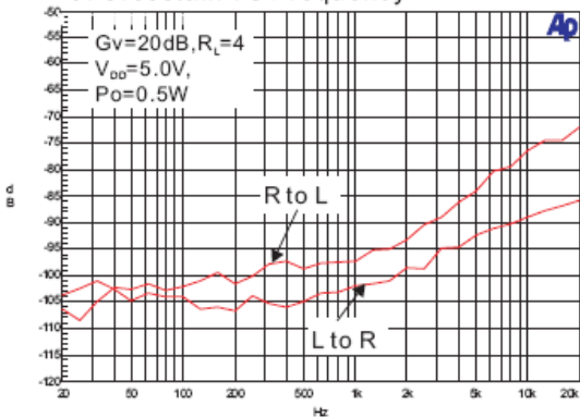
9. Crosstalk VS Frequency
