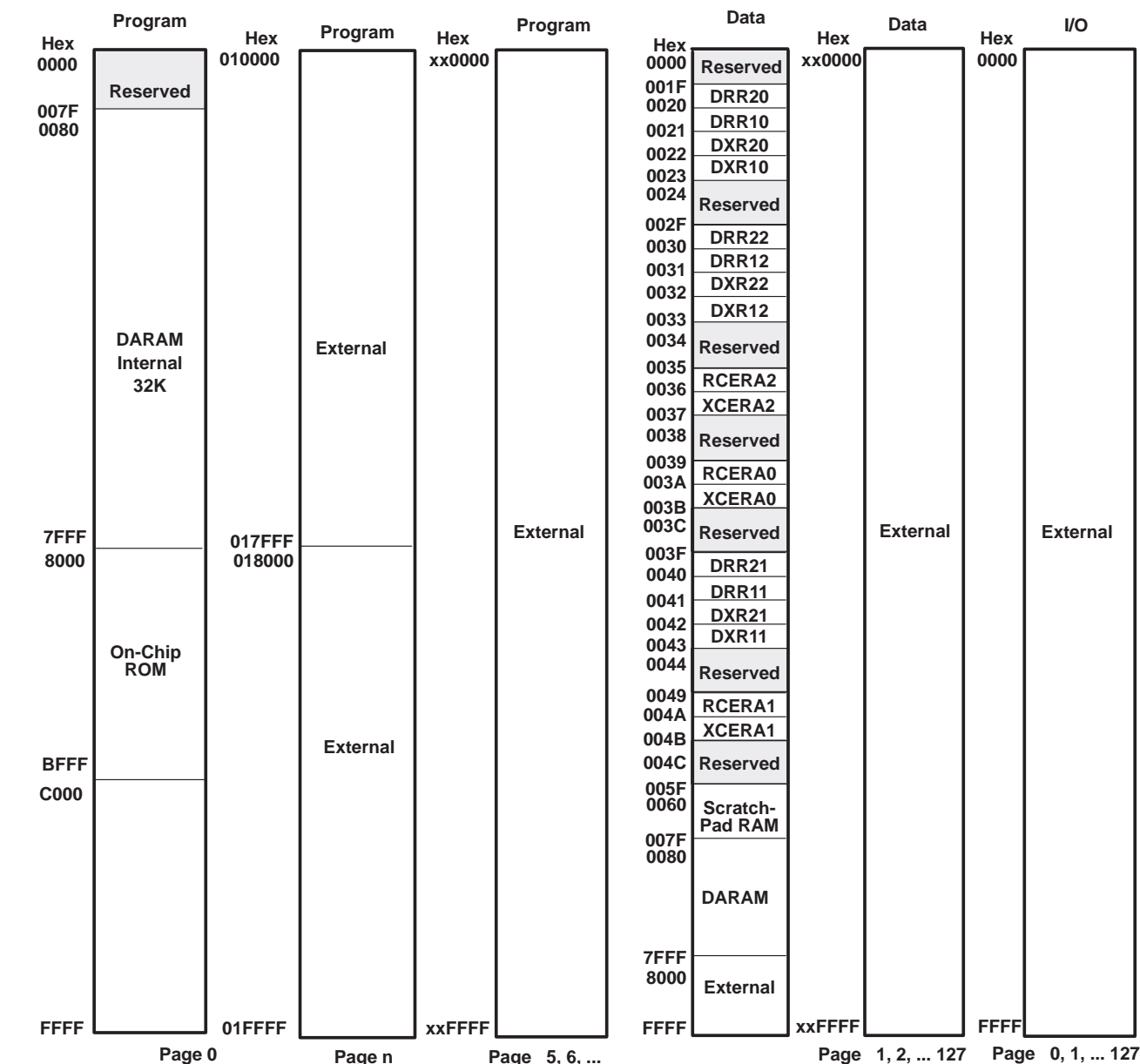
Figure 10. TMS320UC5409 DMA Memory Map
