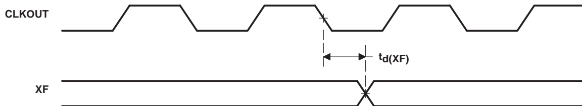
Figure 29. XF Timing
