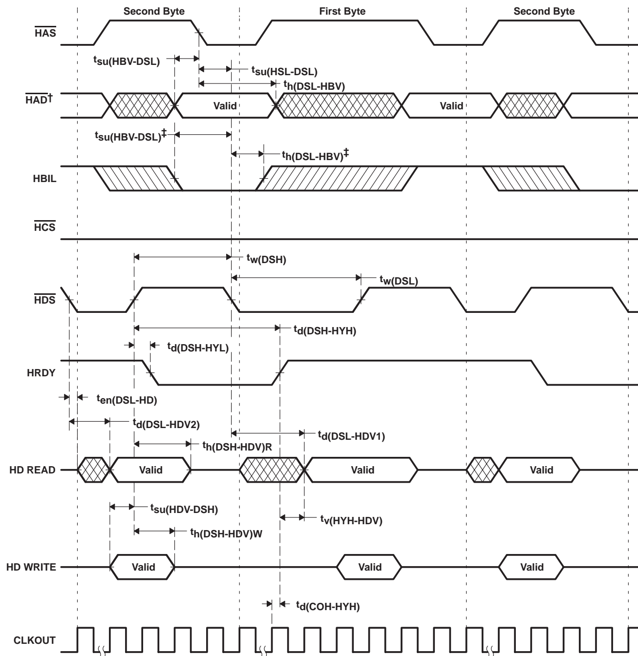
Figure 38. Using \overline{HDS} to Control Accesses ( \overline{HCS} Always Low)
