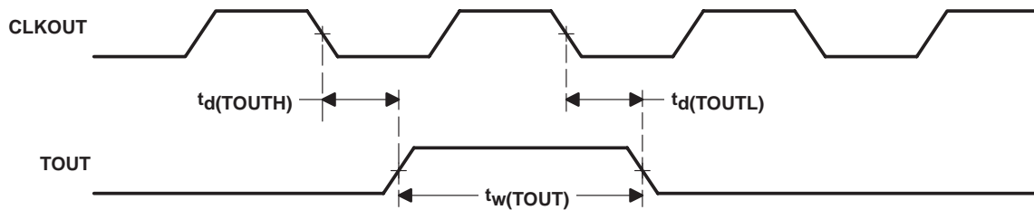
Figure 30. TOUT Timing
