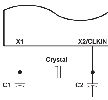
Figure 13. Internal Oscillator With External Crystal
