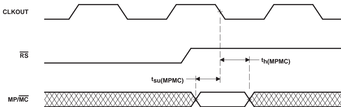
Figure 27. \text{MP}/\overline{\text{MC}} Timing
