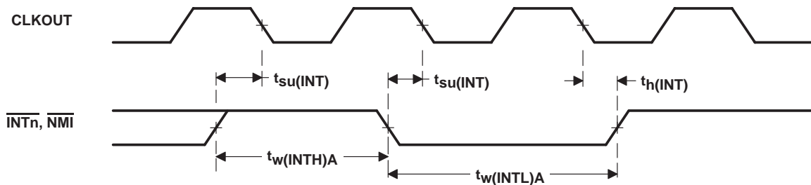
Figure 26. Interrupt Timing
