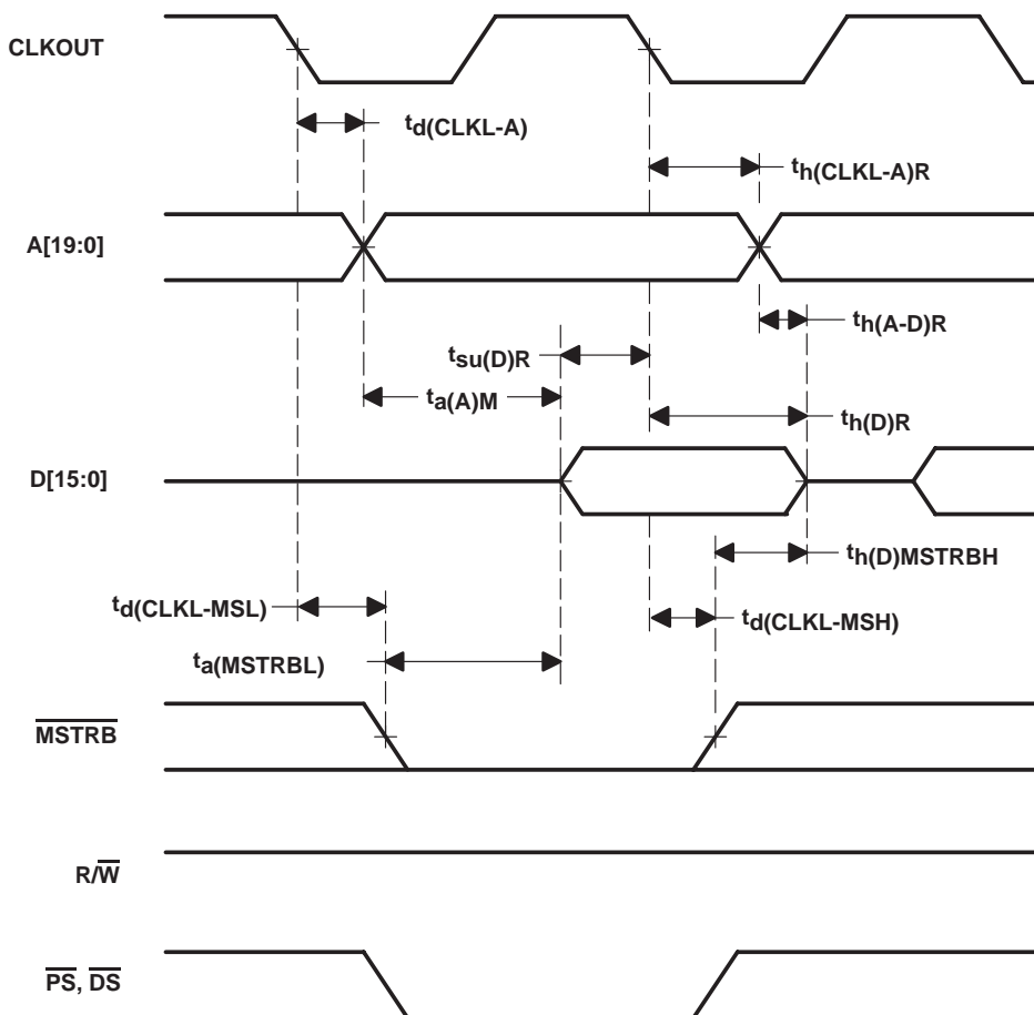
Figure 16. Memory Read ( \overline{\text{MSTRB}} = 0 )
