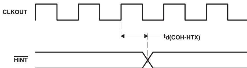
Figure 40. \overline{\text{HINT}} Timing
