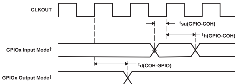
Figure 41. GPIOx † Timings
