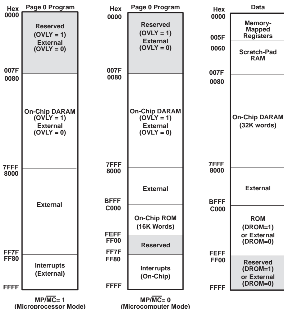
Figure 1. Memory Map
