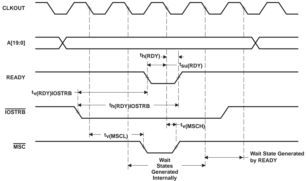
Figure 22. I/O Read With Externally Generated Wait States
