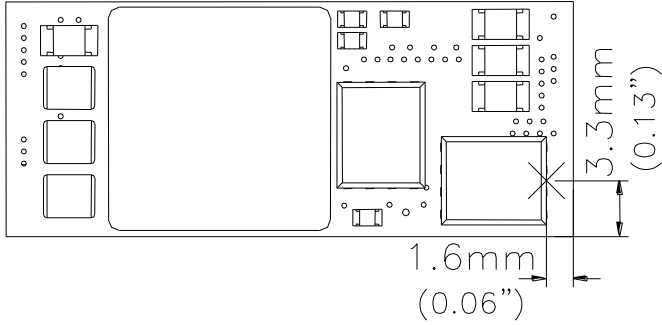
Figure 44: Temperature measurement location
