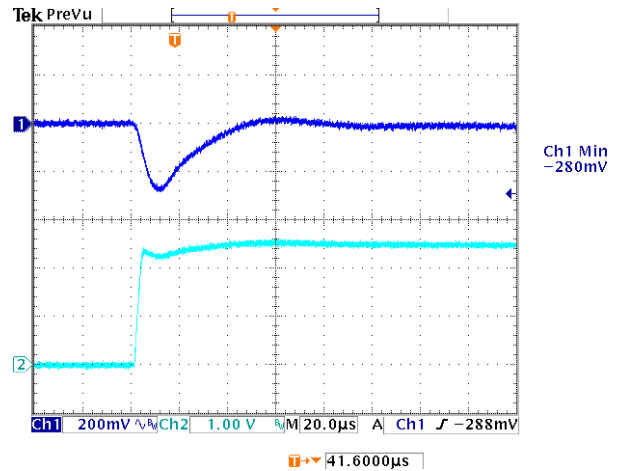
Figure 24: Typical Transient Response to Step Load Change at 2.5A/µS from 50% to 100% of I_o , max at 3.3Vin, 2.5Vout (Cout = 1µF ceramic, 10µF Tantalum)
