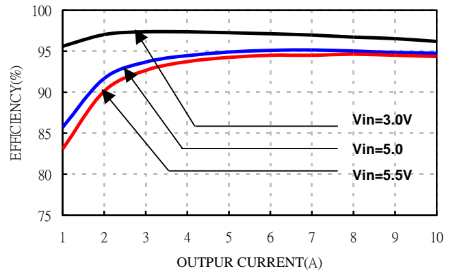
Figure 2: Converter Efficiency vs. Output Current (2.5V out)
