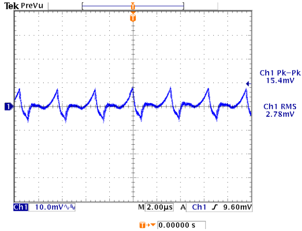
Figure 7: Output ripple & noise at 3.3Vin, 2.5V/10A out
