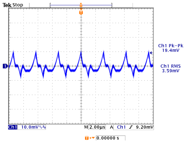
Figure 9: Output ripple & noise at 5Vin, 3.3V/10A out
