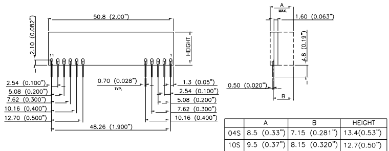
BACK VIEW
