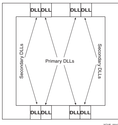
Figure 10: DLL Locations
