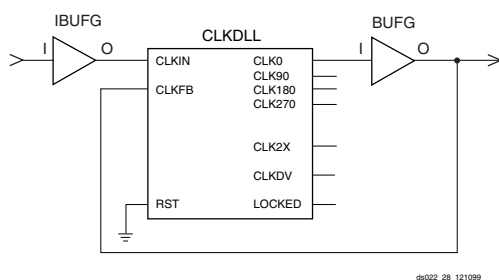
Figure 24: BUFGDLL Schematic
