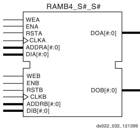
Figure 31: Dual-Port Block SelectRAM+ Memory
