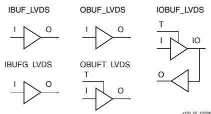
Figure 58: LVDS elements
