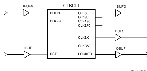
Figure 29: DLL Deskew of Clock and 2x Multiple
