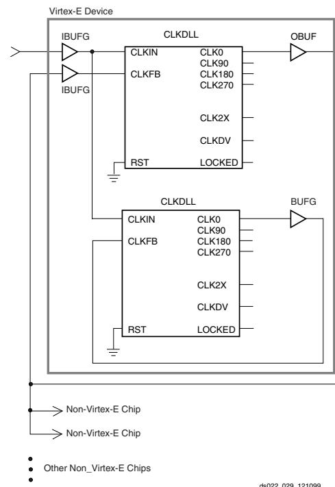
Figure 28: DLL Deskew of Board Level Clock
