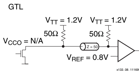
Figure 44: Terminated GTL
