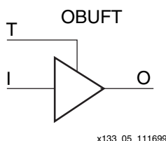
Figure 41: 3-State Output Buffer Symbol (OBUFT)
