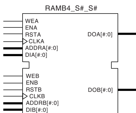
Figure 3: Dual-Port Block SelectRAM
