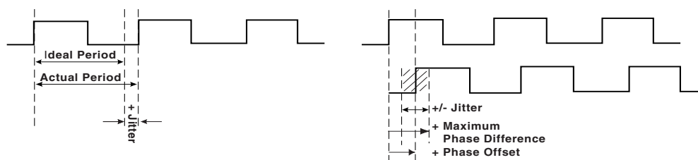
Figure 4: DLL Timing Waveforms
