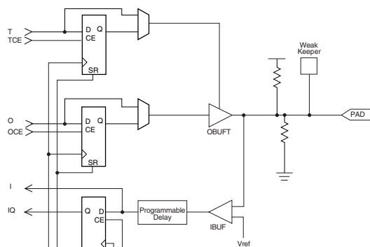
Figure 1: Virtex-E Input/Output Block (IOB)
