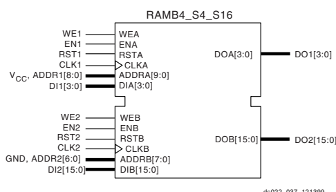
Figure 36: 512 x 4 RAM and 128 x 16 RAM
