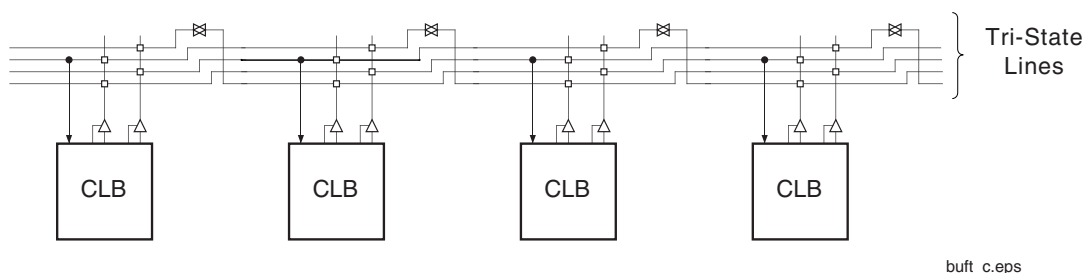
Figure 8: BUFT Connections to Dedicated Horizontal Bus Lines
