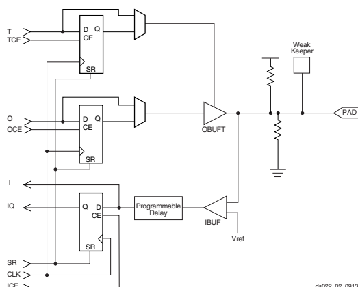
Figure 2: Virtex-E Input/Output Block (IOB)
