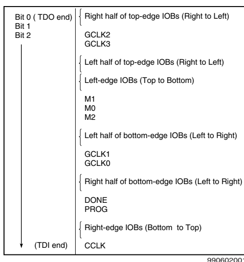
Figure 12: Boundary Scan Bit Sequence
