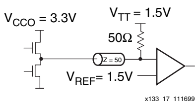
Figure 53: Terminated CTT
