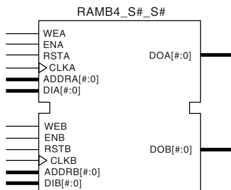
Figure 6: Dual-Port Block SelectRAM
