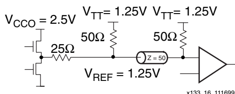
Figure 52: Terminated SSTL2 Class II
