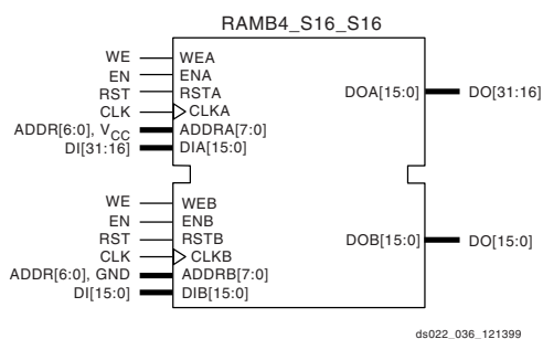
Figure 35: Single Port 128 x 32 RAM
