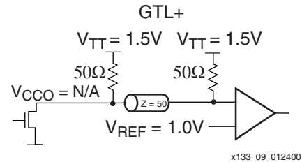
Figure 45: Terminated GTL+
