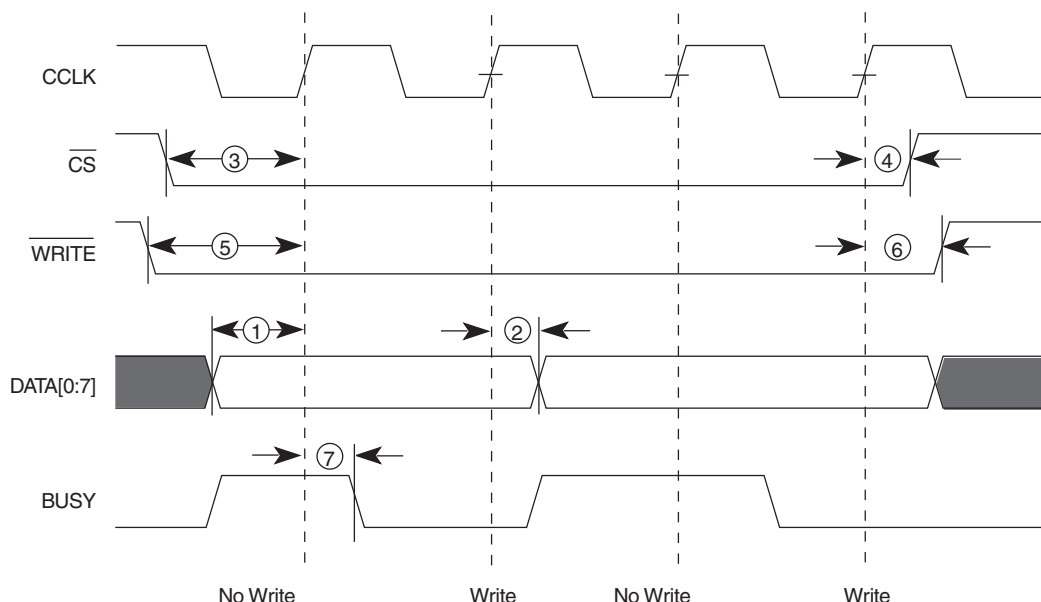
Figure 17: Write Operations
