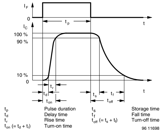
Fig. 3 - Switching Times
