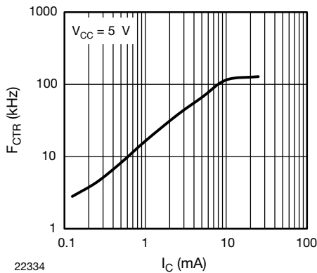
Fig. 12 - F_{CTR} vs. I_C (saturated) (mA)
