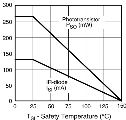
Fig. 2 - Derating Diagram
