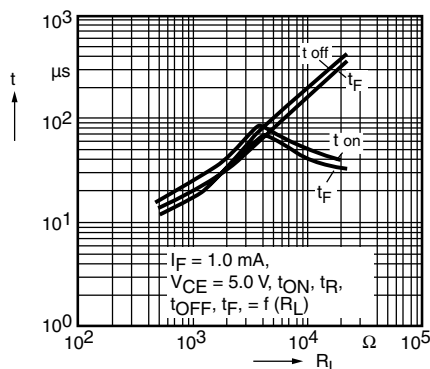
Fig. 2 - Switching Times
