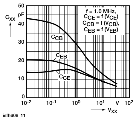
Fig. 11 - Transistor Capacitance
