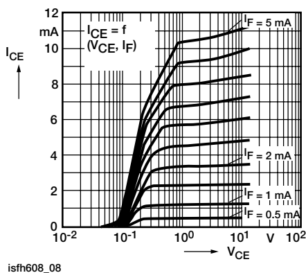
Fig. 8 - Output Characteristics
