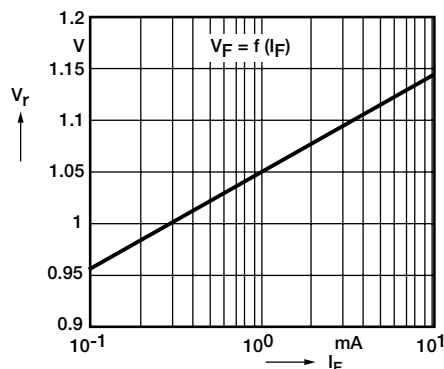
Fig. 5 - Diode Forward Voltage (typ.)
