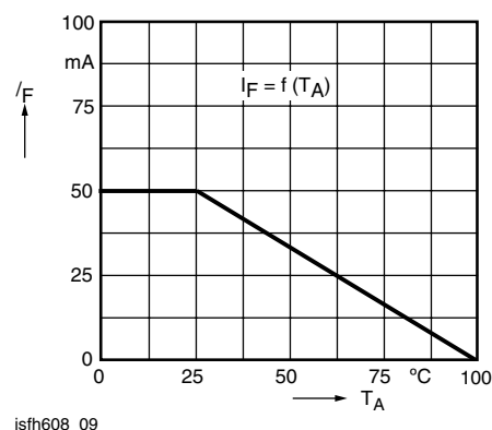
Fig. 9 - Permissible Forward Current Diode
