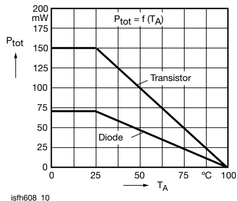
Fig. 10 - Permissible Power Dissipation for Transistor and Diode
