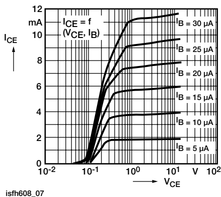
Fig. 7 - Output Characteristics
