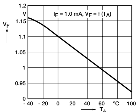
Fig. 6 - Diode Forward Voltage (typ.)
