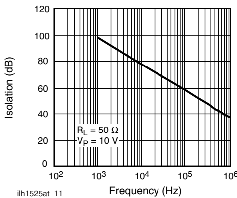
Fig. 12 - Output Isolation
