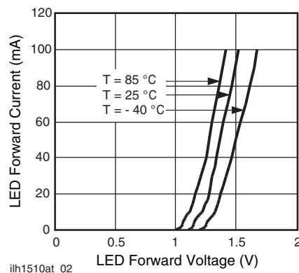
Fig. 3 - LED Forward Current vs. LED Forward Voltage
