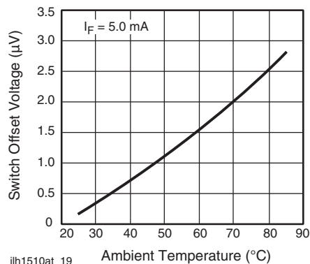
Fig. 20 - Switch Offset Voltage vs. Temperature
