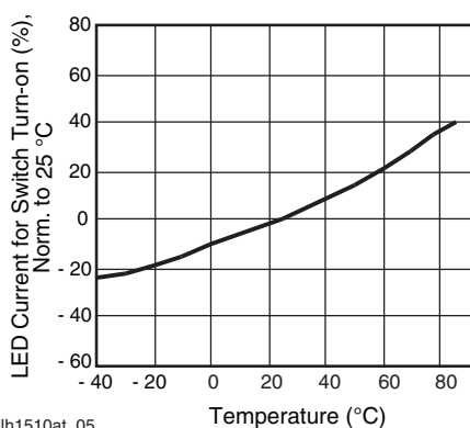
Fig. 6 - LED Current for Switch Turn-on vs. Temperature
