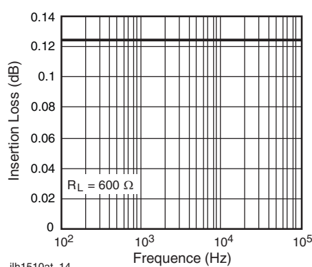
Fig. 15 - Insertion Loss vs. Frequency
