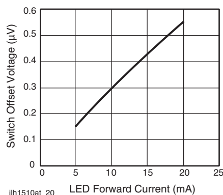
Fig. 21 - Switch Offset Voltage vs. LED Current
