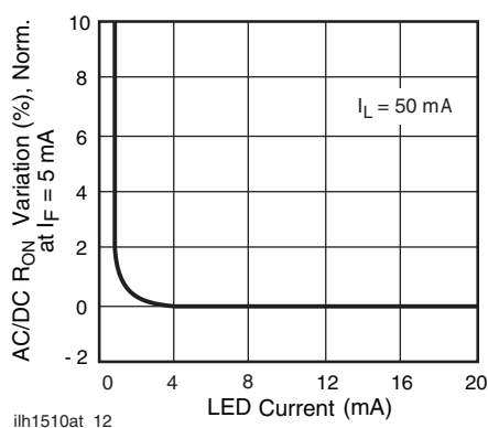
Fig. 13 - Variation in On-Resistance vs. LED Current
