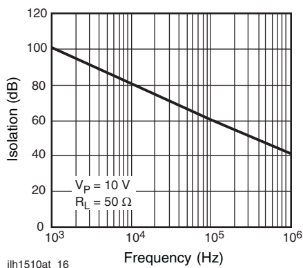
Fig. 17 - Output Isolation
