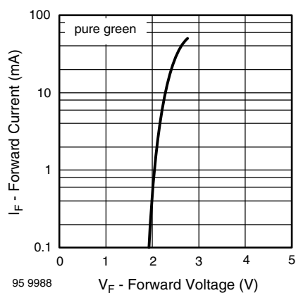
Fig. 25 - Forward Current vs. Forward Voltage
