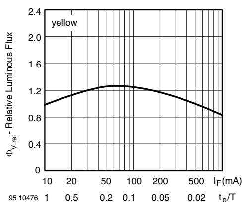
Fig. 17 - Relative Luminous Flux vs. Forward Current/Duty Cycle
