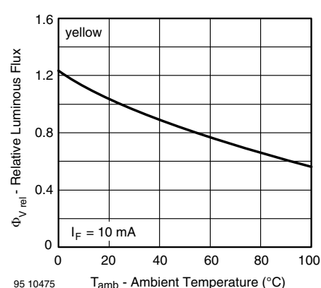
Fig. 18 - Relative Luminous Flux vs. Ambient Temperature
