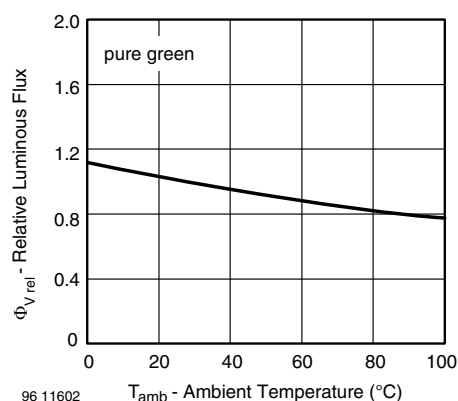
Fig. 28 - Relative Luminous Flux vs. Ambient Temperature
