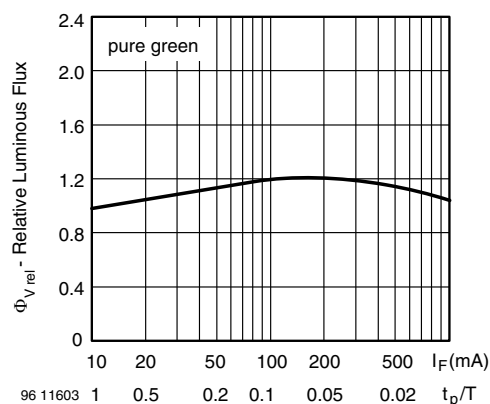
Fig. 27 - Relative Luminous Flux vs. Forward Current/Duty Cycle
