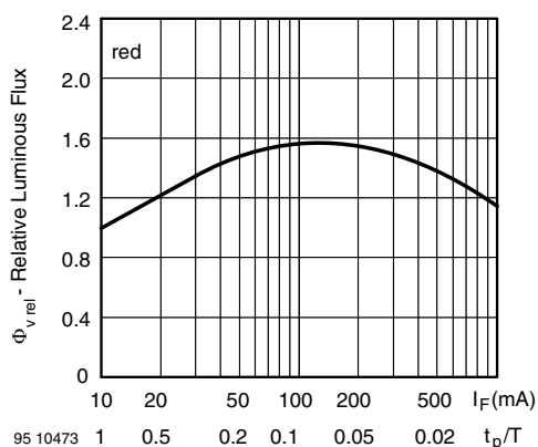
Fig. 7 - Relative Luminous Flux vs. Forward Current/Duty Cycle
