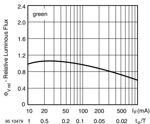
Fig. 23 - Relative Luminous Flux vs. Forward Current/Duty Cycle
