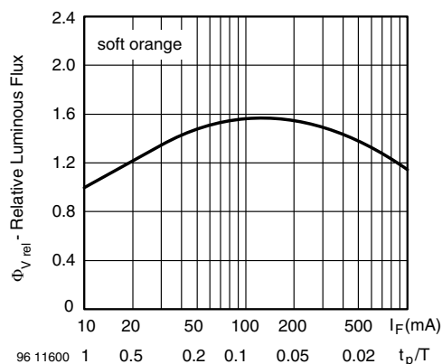
Fig. 11 - Relative Luminous Flux vs. Forward Current/Duty Cycle
