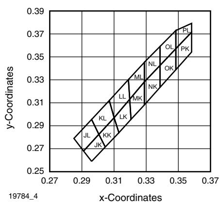
Fig. 9 - Coordinates of Colorgroups
