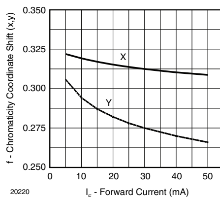
Fig. 6 - Chromaticity Coordinate Shift vs. Forward Current
