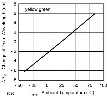
Fig. 32 - Change of Dominant Wavelength vs. Ambient Temperature
