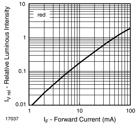
Fig. 11 - Relative Luminous Flux vs. Forward Current
