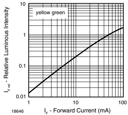
Fig. 29 - Relative Luminous Flux vs. Forward Current
