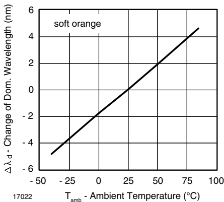
Fig. 21 - Change of Dominant Wavelength vs. Ambient Temperature
