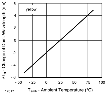
Fig. 26 - Change of Dominant Wavelength vs. Ambient Temperature
