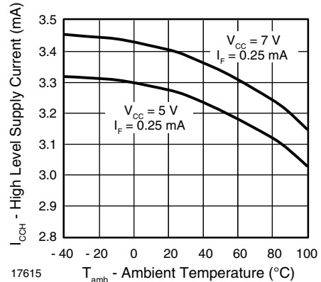
Fig. 7 - High Level Supply Current vs. Ambient Temperature
