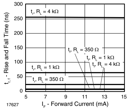
Fig. 19 - Rise and Fall Time vs. Forward Current
