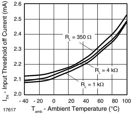
Fig. 9 - Input Threshold off Current vs. Ambient Temperature
