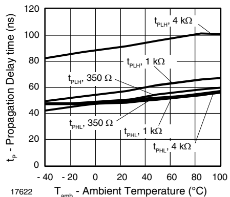
Fig. 14 - Propagation Delay vs. Ambient Temperature
