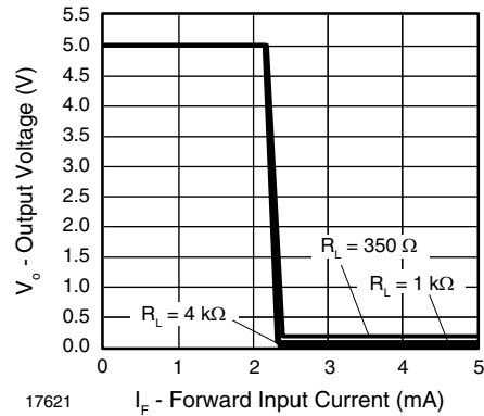
Fig. 13 - Output Voltage vs. Forward Input Current
