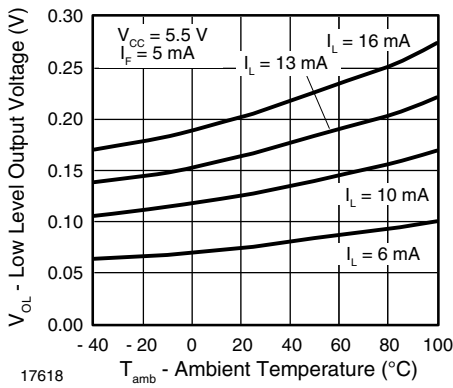
Fig. 10 - Low Level Output Voltage vs. Ambient Temperature
