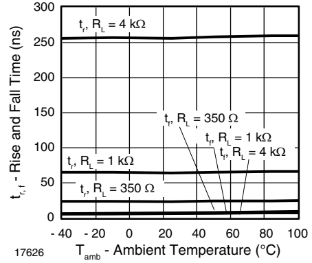
Fig. 18 - Rise and Fall Time vs. Ambient Temperature
