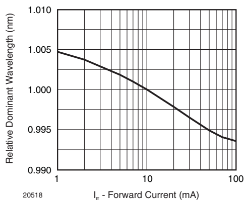
Fig. 3 - Relative Dominant Wavelength vs. Forward Current
