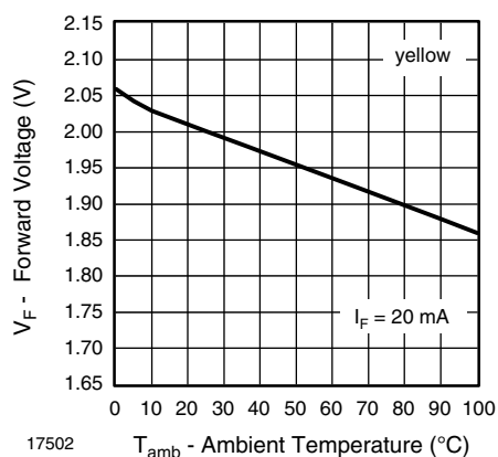
Fig. 17 - Forward Voltage vs. Ambient Temperature
